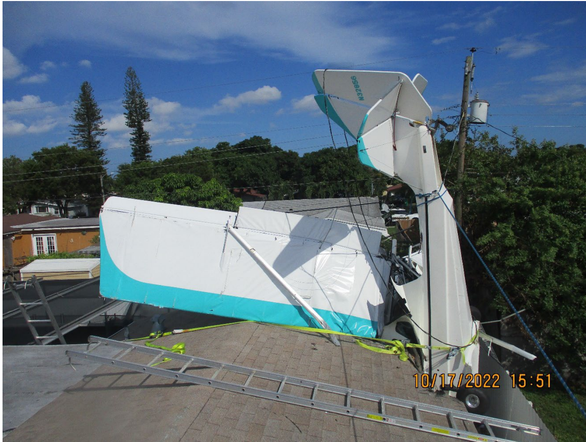
Photograph 2 - View of aircraft wreckage on house rooftop (Courtesy of FAA)
