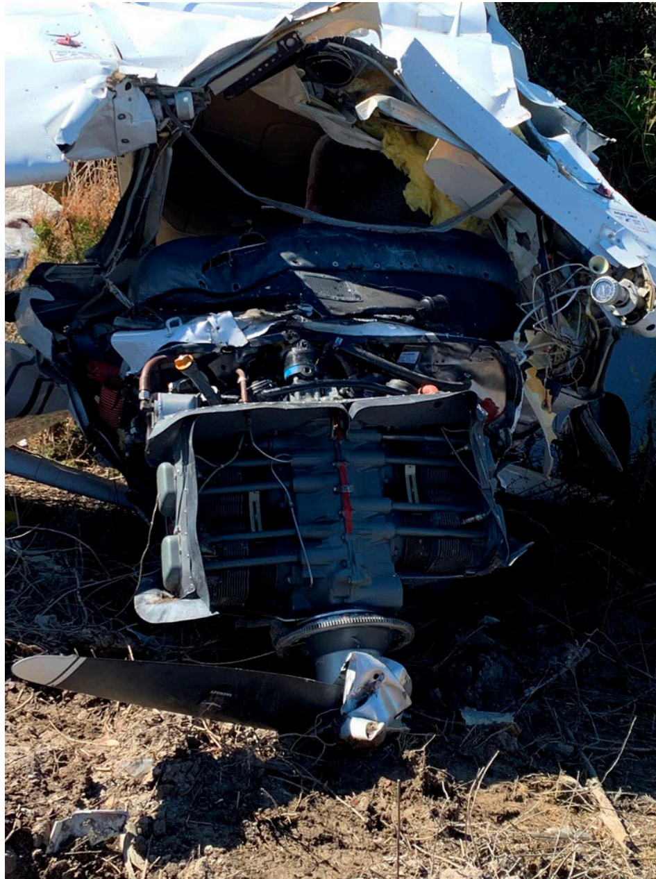
Photo 5 – Front View of Engine on Airplane
