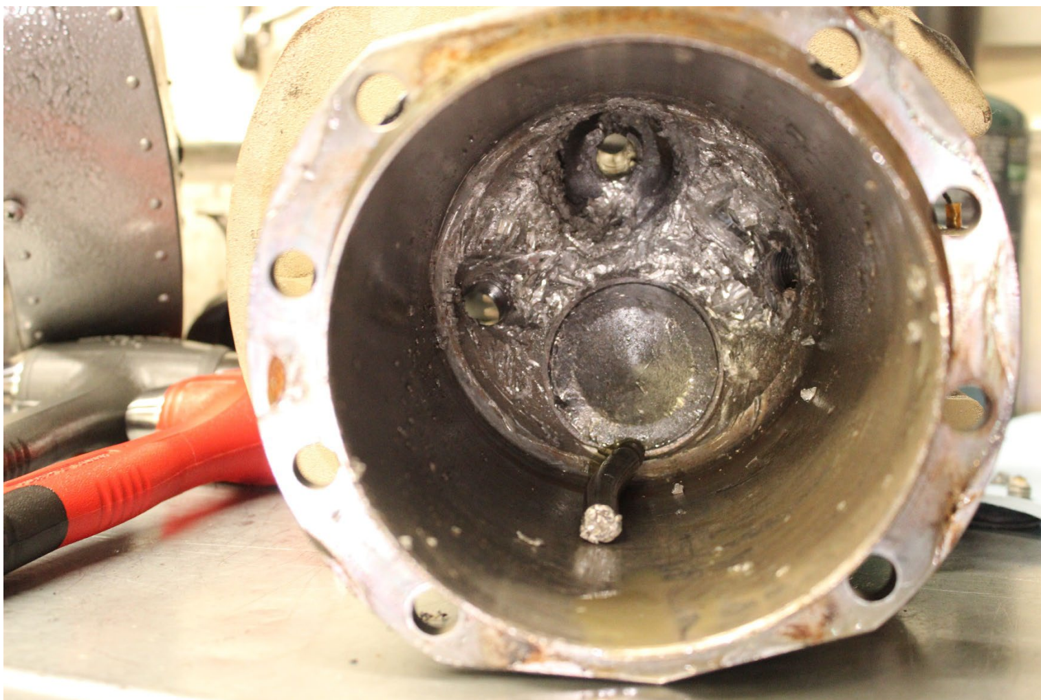
Photograph 2 - View of damage to No. 1 cylinder.
