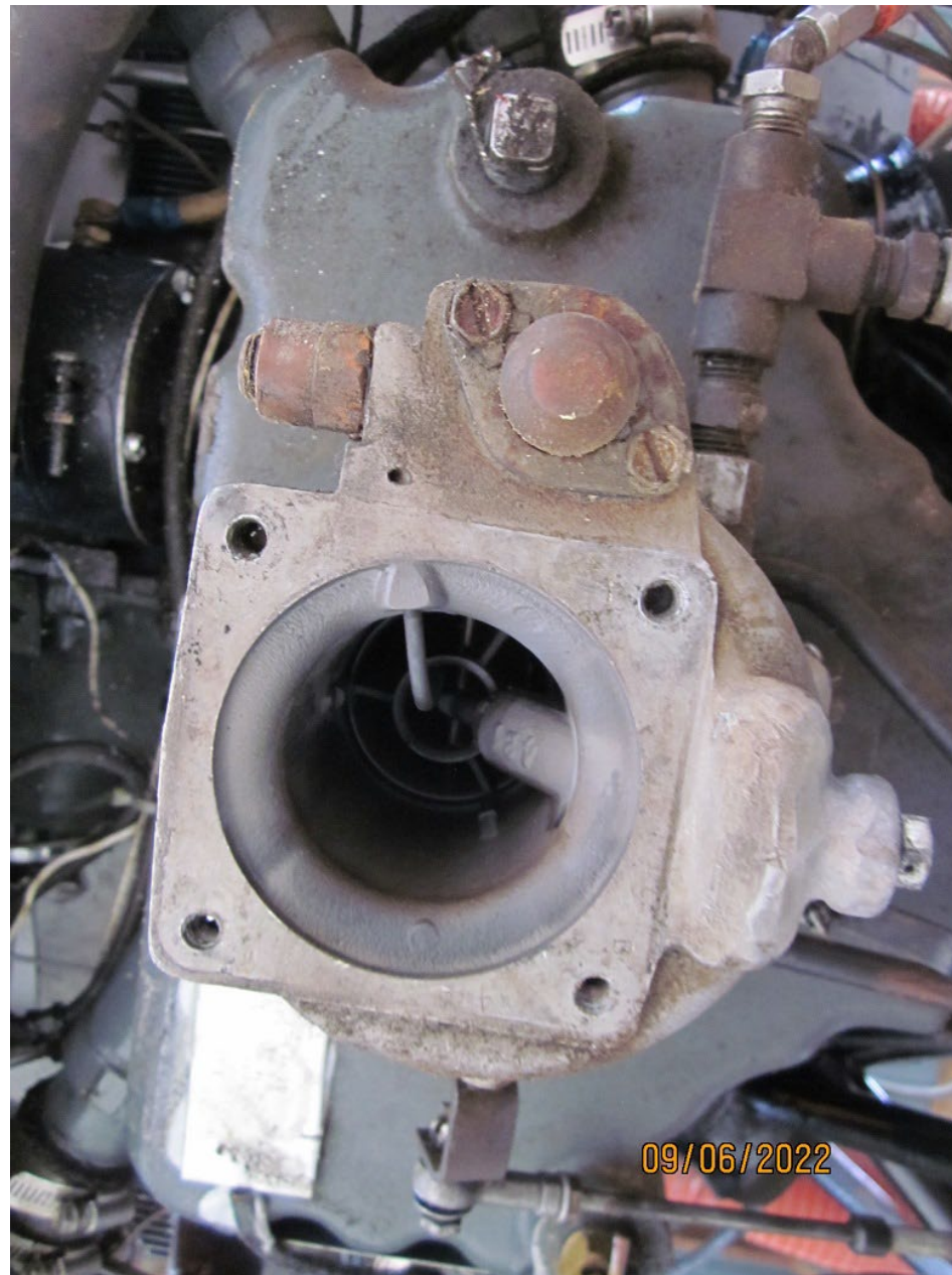
Photo 5 – Carburetor (Photo Courtesy of FAA)
