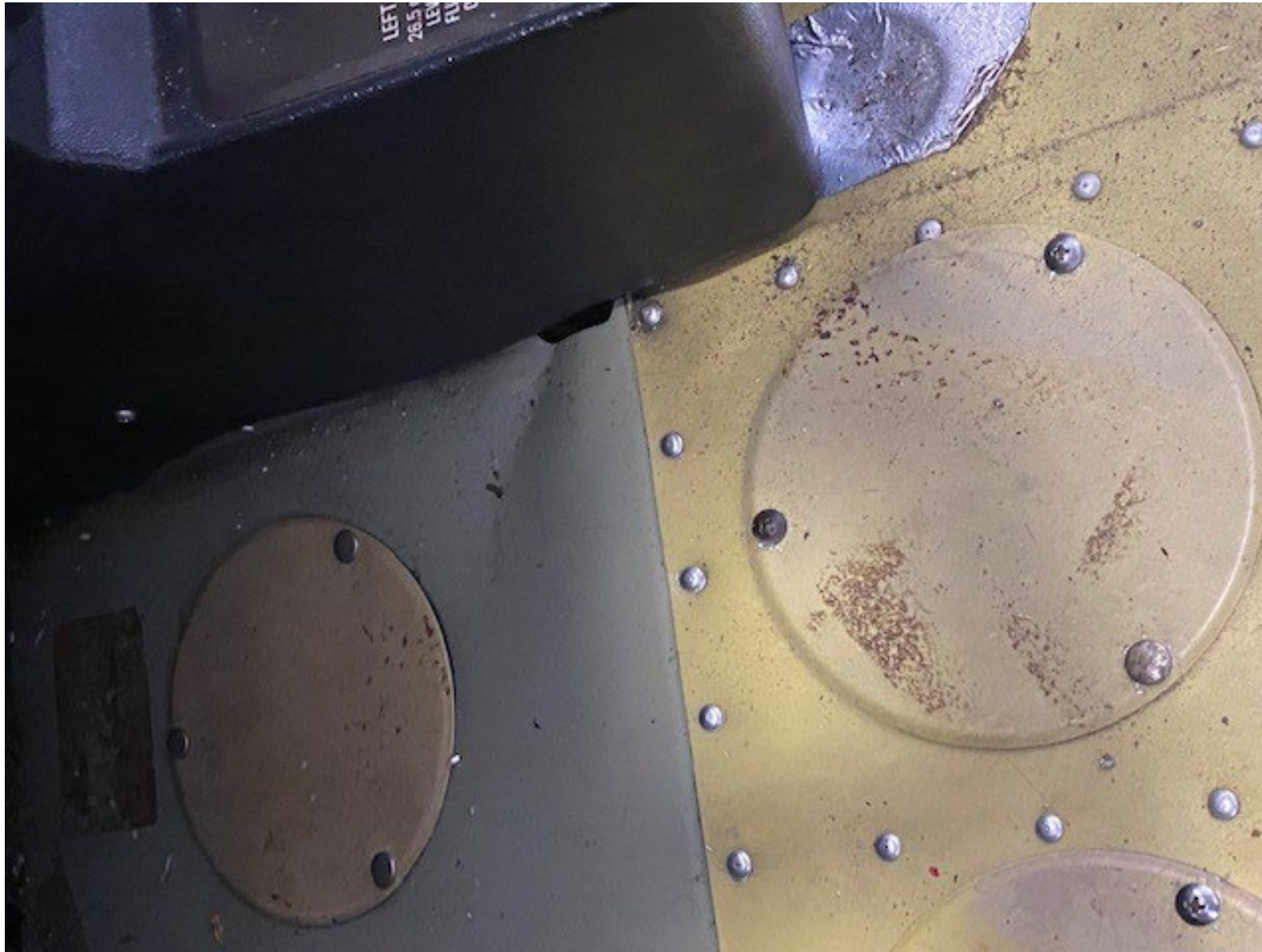
Photo 2: Wrinkling of the floorboard in the cockpit left side of pedestal (Photo Courtesy of FAA)
