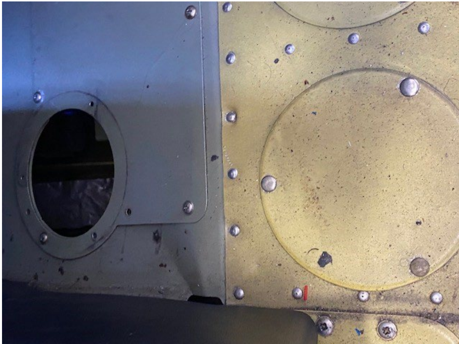
Photo 3: Wrinkling of the floorboard in the cockpit right side of pedestal (Photo Courtesy of FAA)
