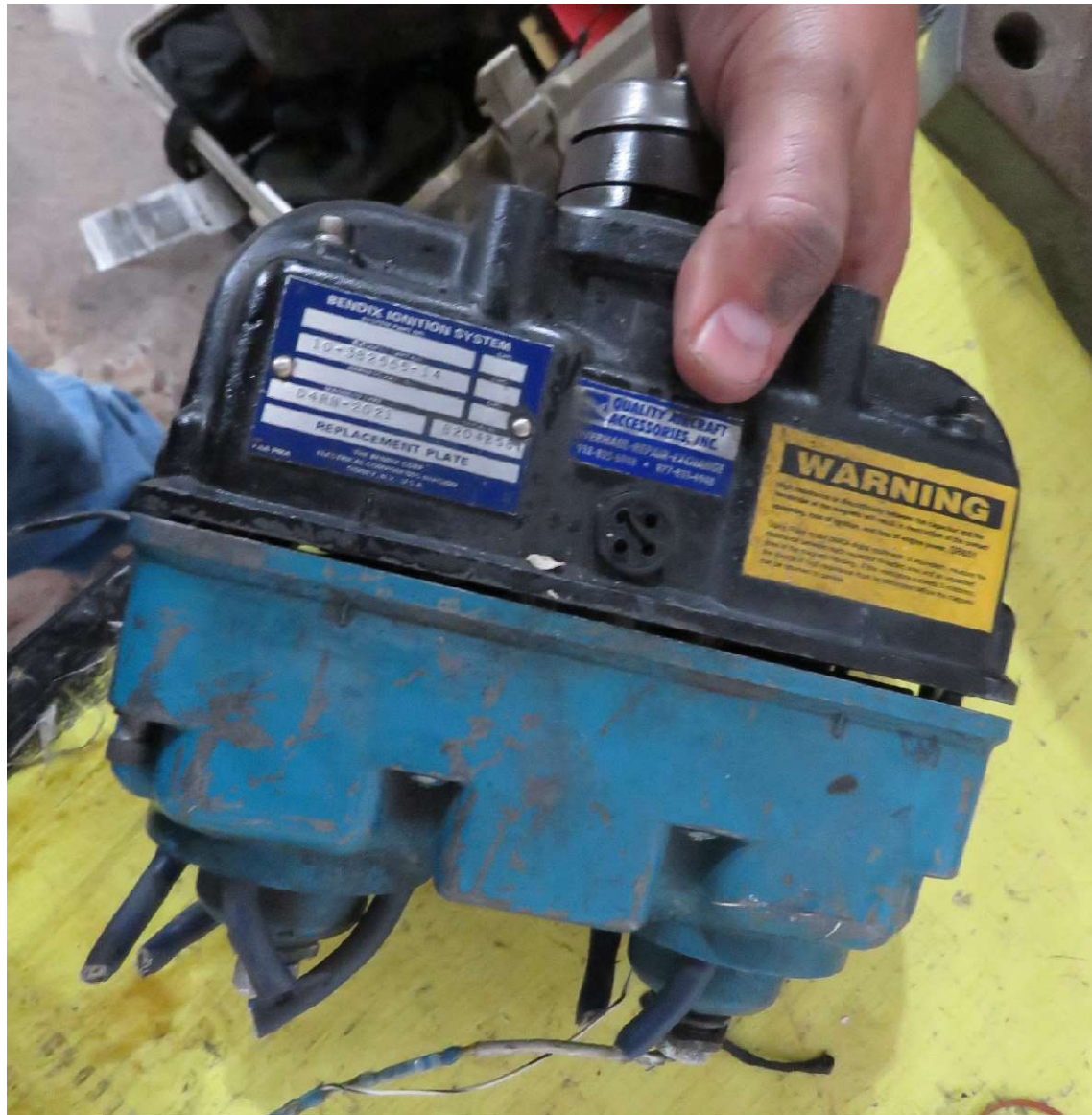
Photo 5 – View of Magneto (Photo Courtesy of Lycoming Engines)
