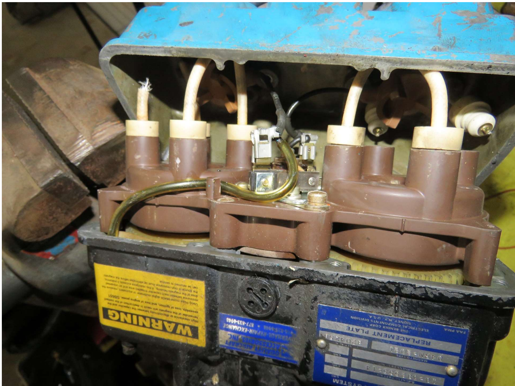
Photo 6 – View of Magneto with Cover Removed (Photo Courtesy of Lycoming Engines)
