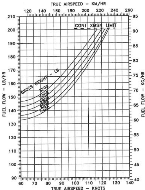
Figure 3-1. Fuel flow (Sheet 3 of 24)
