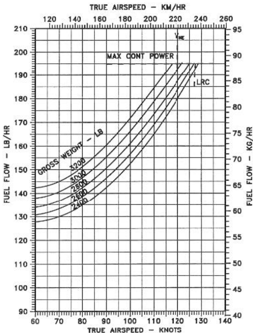
Figure 3-1. Fuel flow (Sheet 6 of 24)
