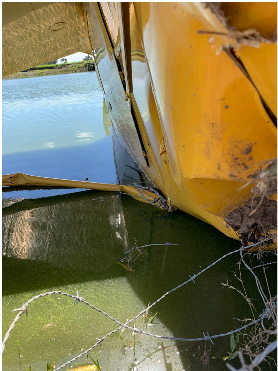
Photo 2 – Forward Right Fuselage And Right Wing Strut Damage (Photo Courtesy of FAA)
