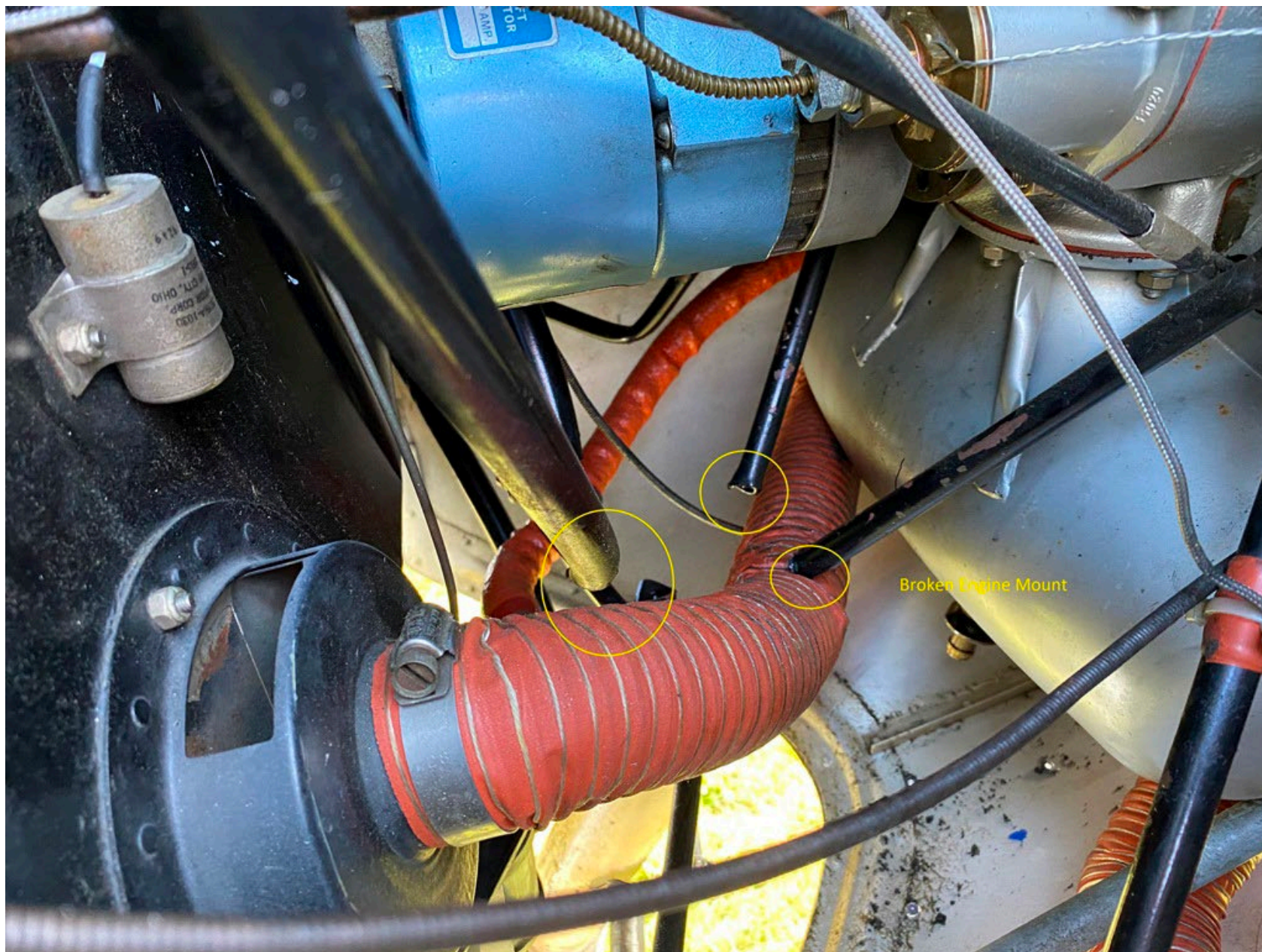
Photo 2 – Broken Engine Mounts (FAA)
