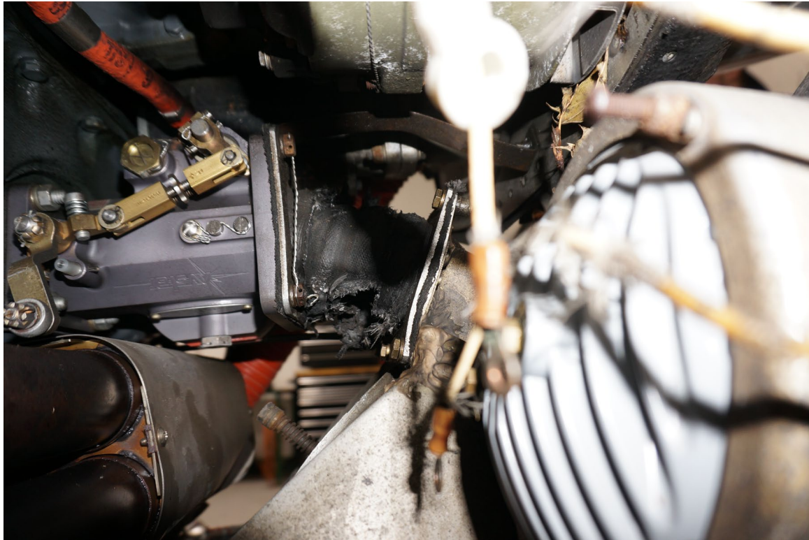
Photograph 5 - Deteriorated fuel injector airbox boot
