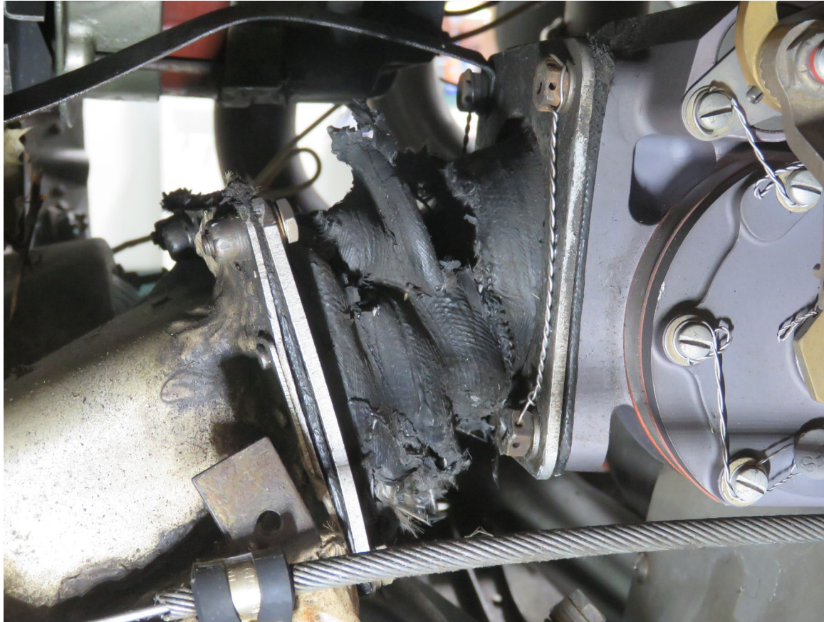
Photograph 4 - Deteriorated fuel injector airbox boot (Courtesy of Lycoming)
