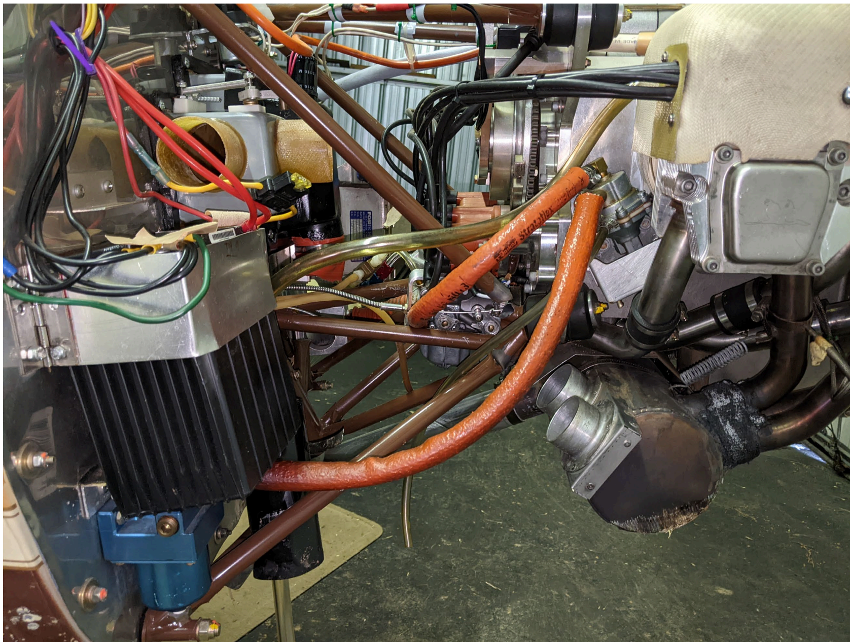
Photo 5 – Digital Photograph From Airport Manager. Right Side View of the Aft Portion of the Engine and Engine Firewall Following Recovery.
