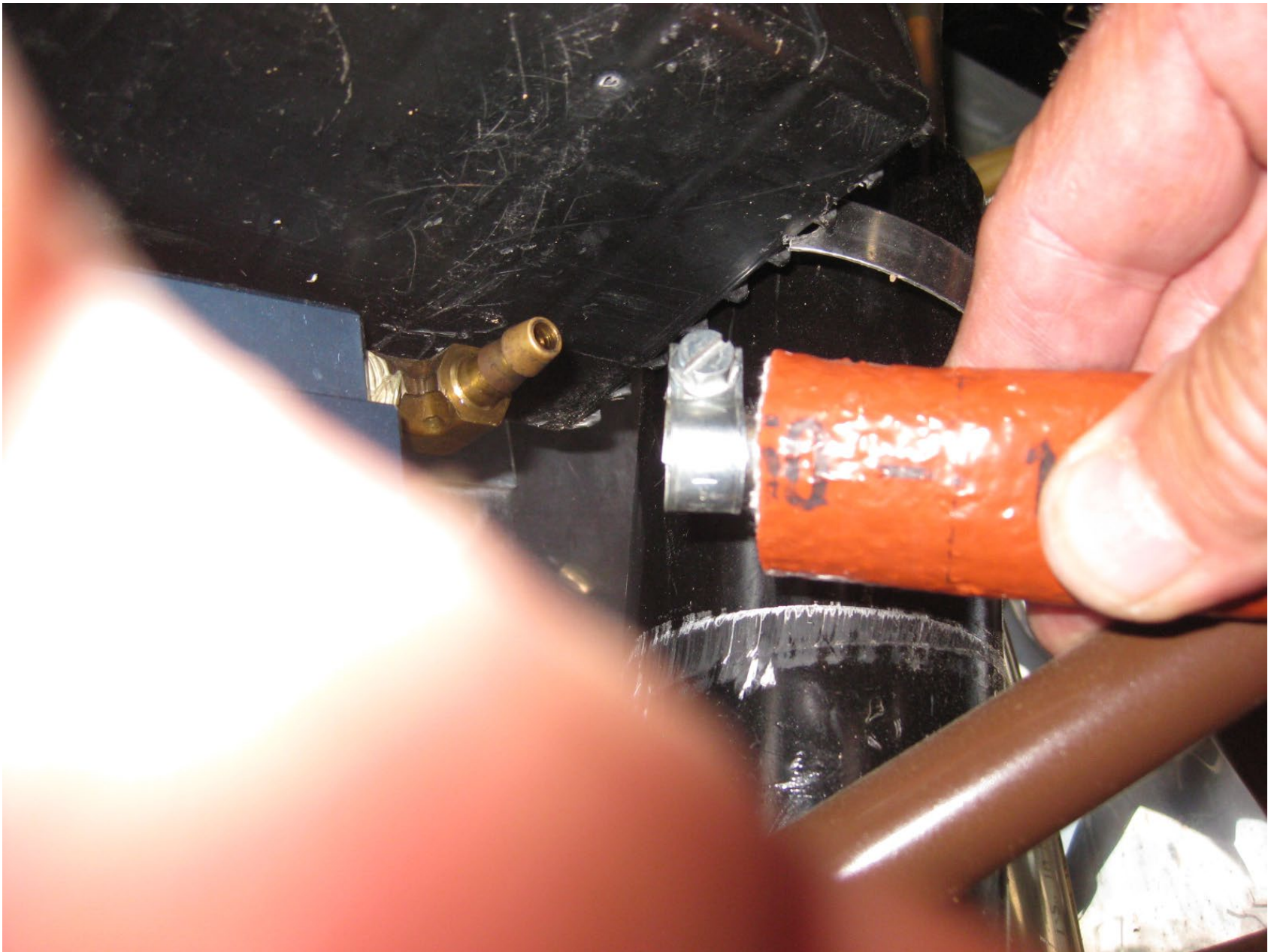
Photo 4 – FAA Digital Photograph. View of the Loose Hose at the Outlet of the Gascolator.
