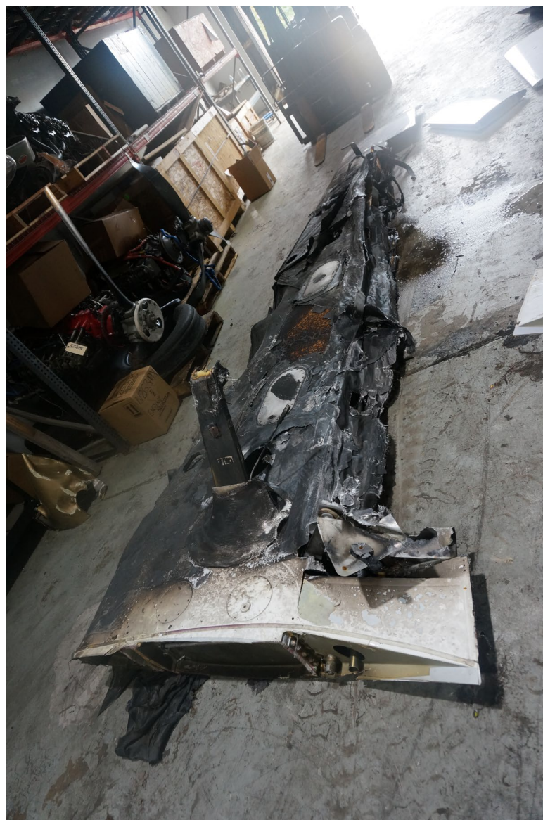
Photograph 4 - Left Wing
