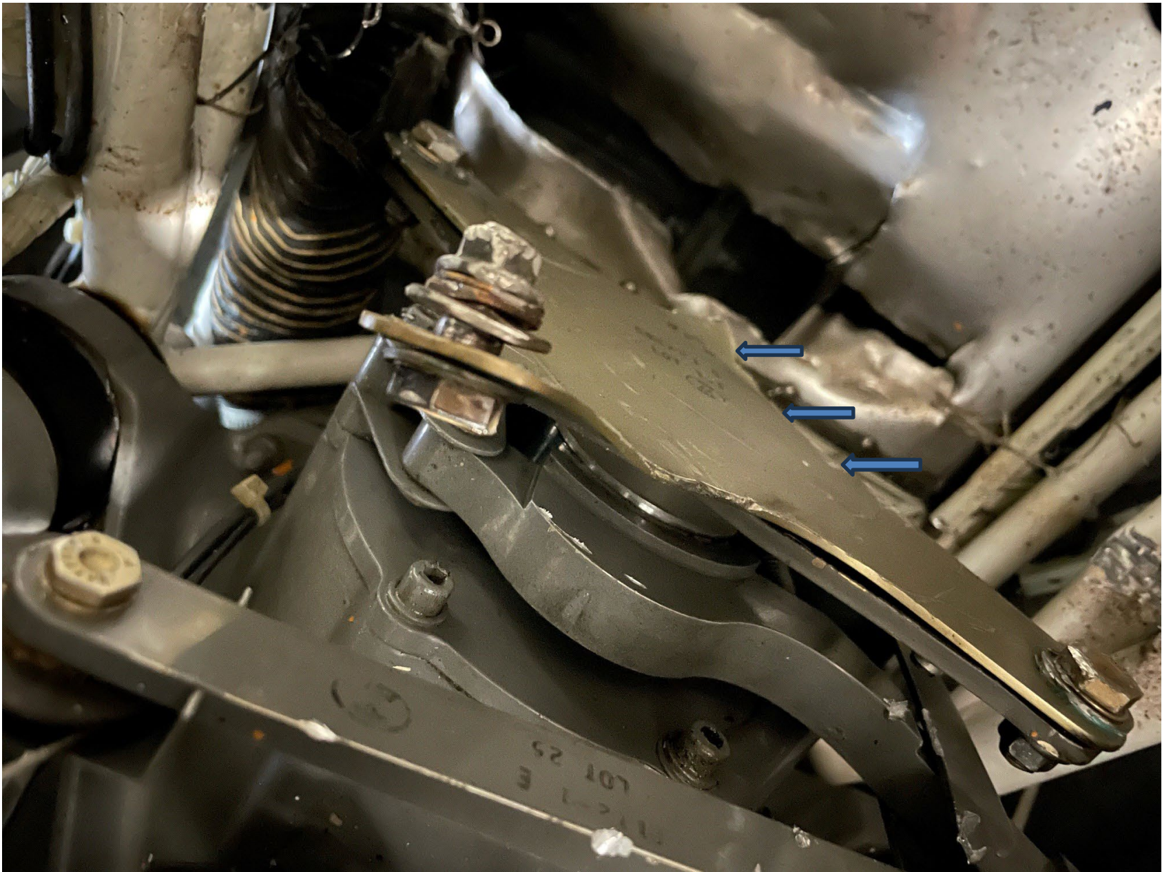
Photo 4 – View of Fractured Flex Plate Coupling (Operator)
