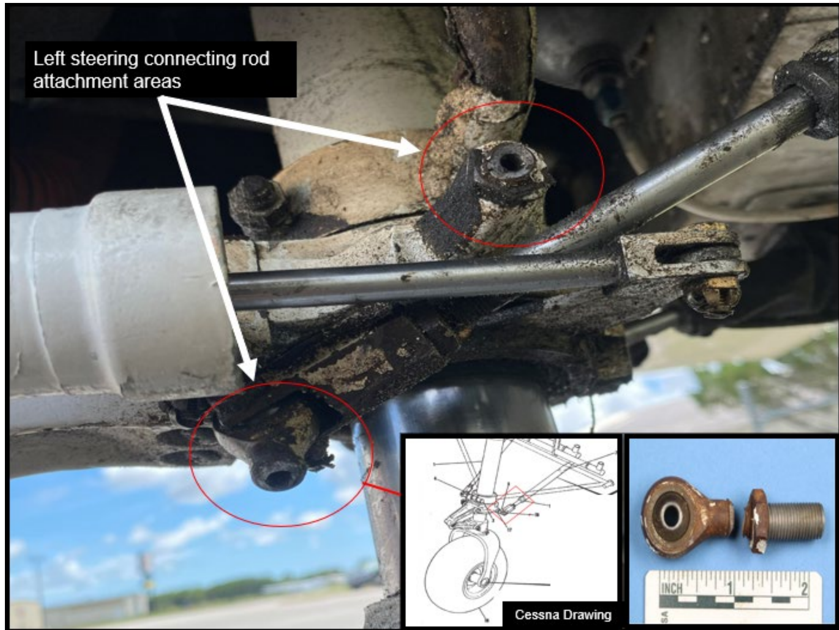
Photo 6: Overview of the left steering connecting rod (Figure from report)
