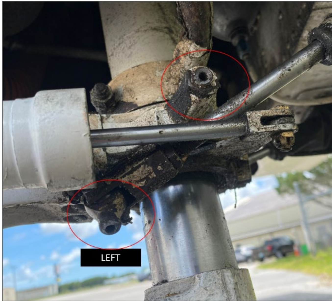
Photo 4: Overview of the left steering connecting rod (Photo Courtesy of FAA)
