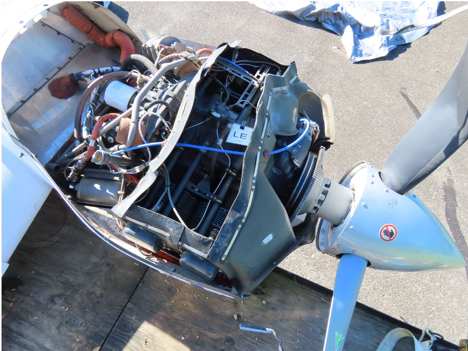
Photograph 5 - Left Engine (Courtesy of Lycoming Engines)
