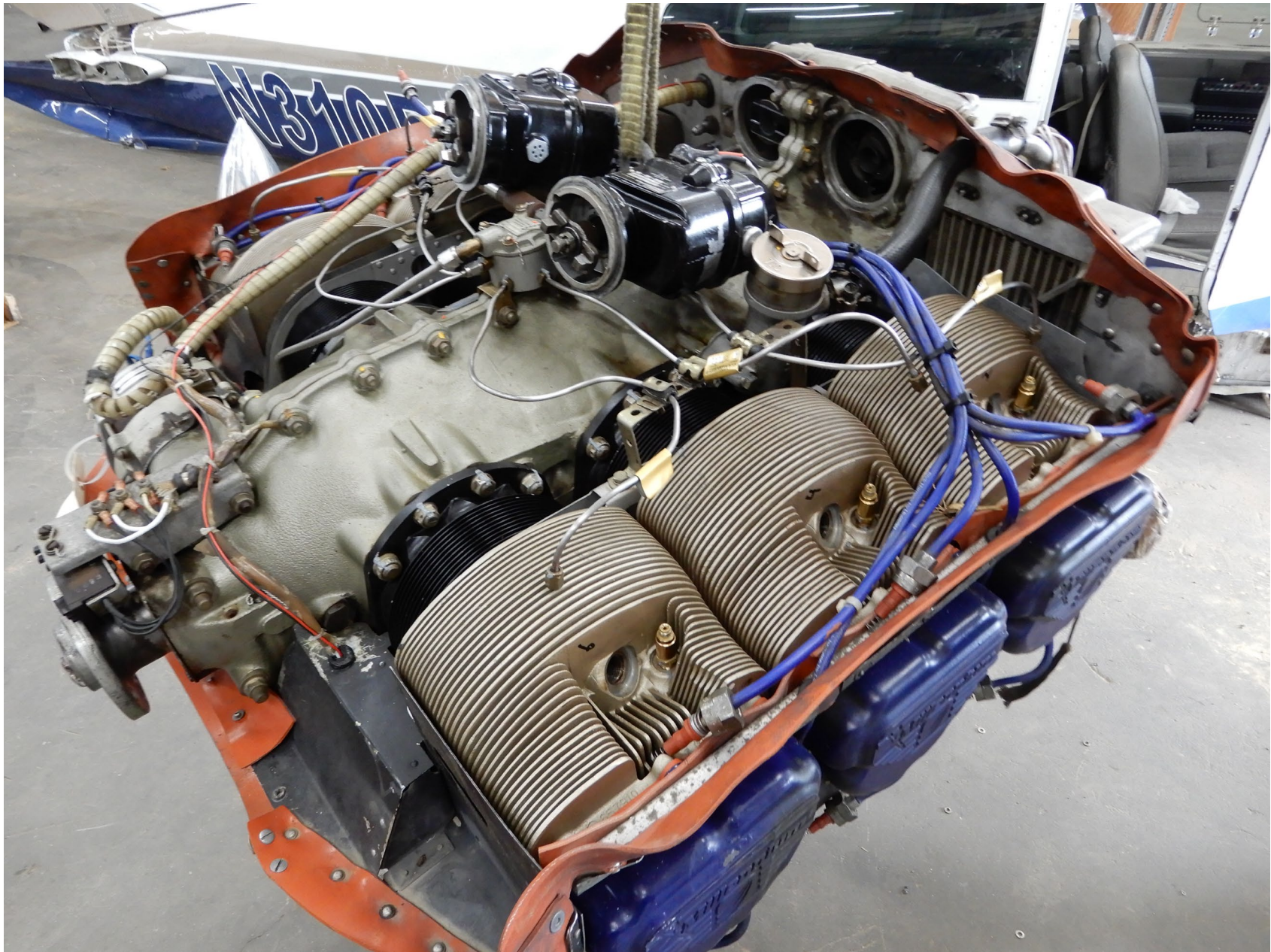
Photo 8 - Right Engine (NTSB Photo)
