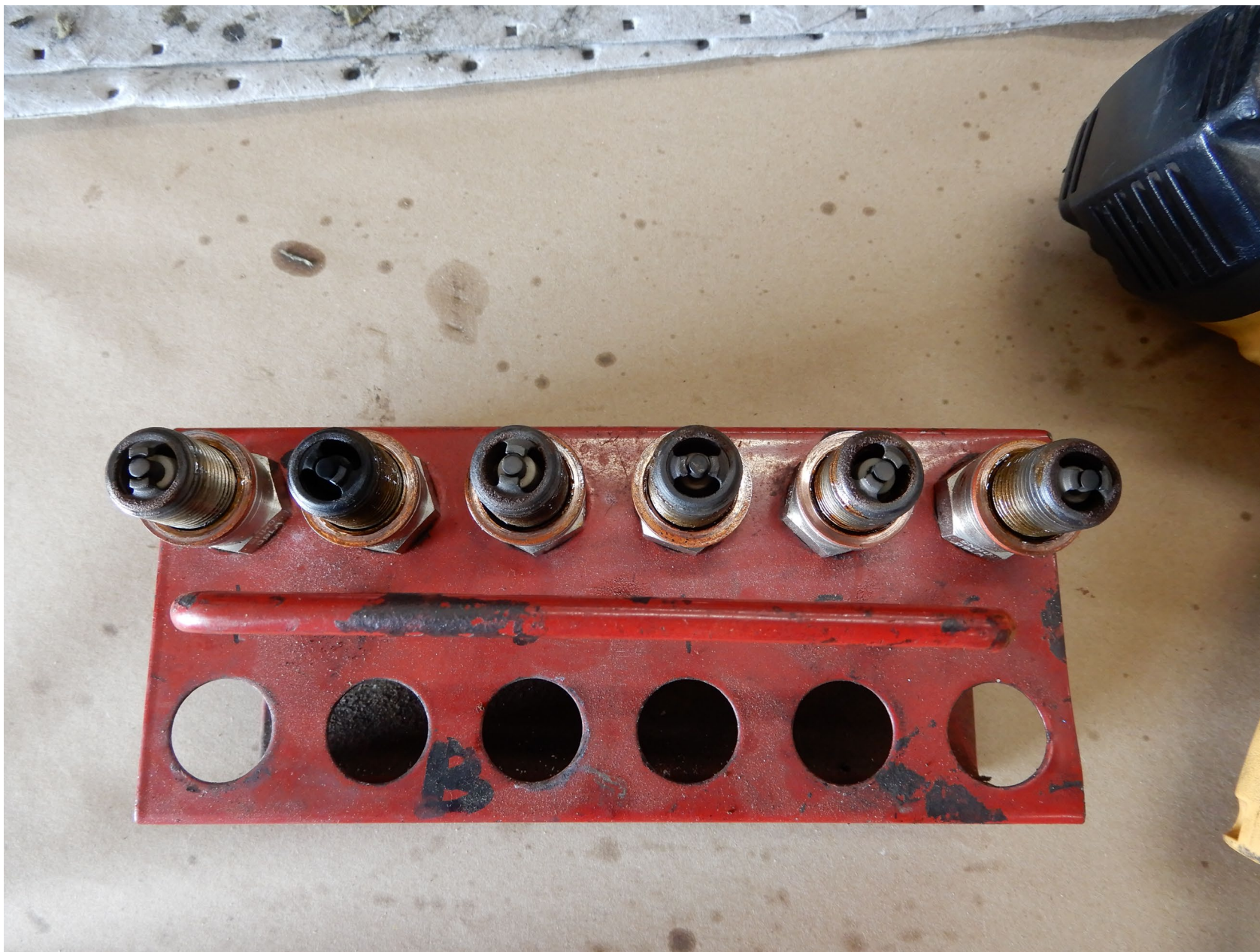
Photo 9 - Right Engine Spark Plugs (NTSB Photo)
