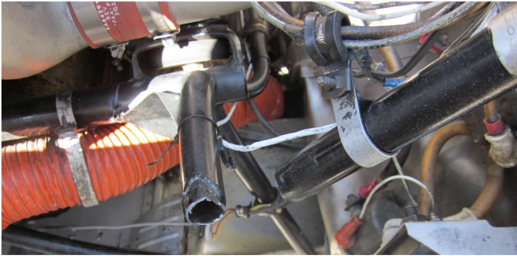
Photograph 4 – Accident airplane, broken engine mount.
