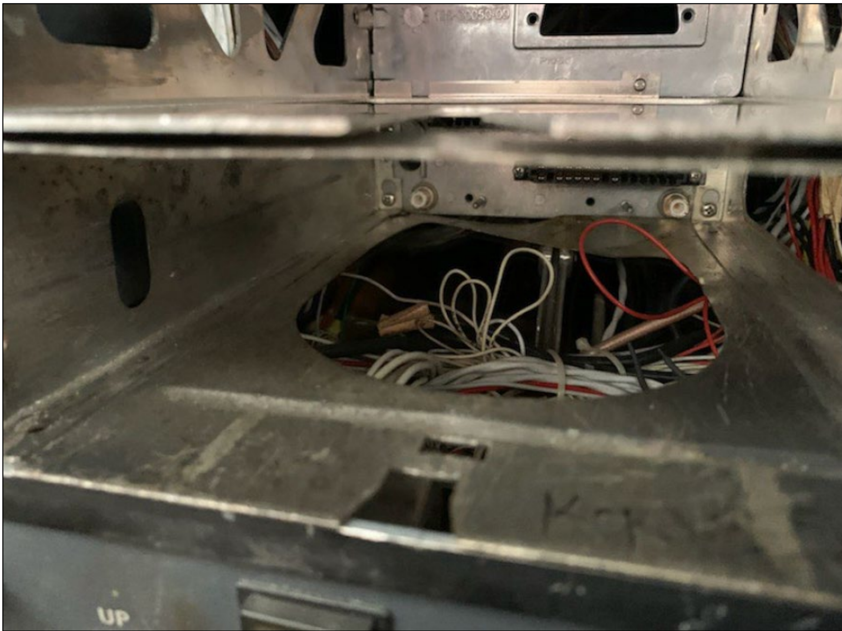
Photo 7: View of the KX-155 avionics tray (Photo Courtesy of FAA)
