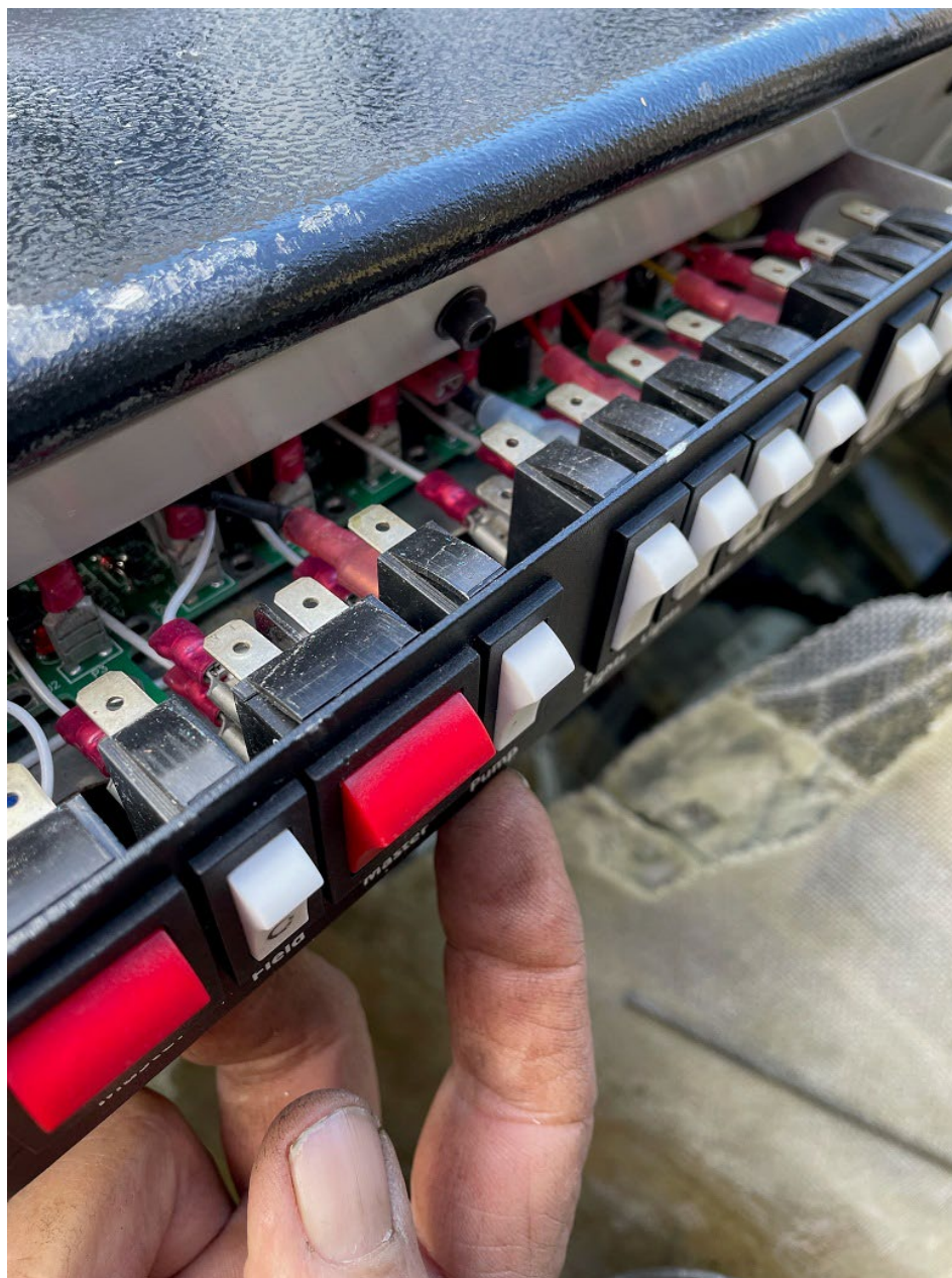
Photo 7 – Reconnected Electric Boost Pump Wiring (Photo Courtesy of Airport Manager)
