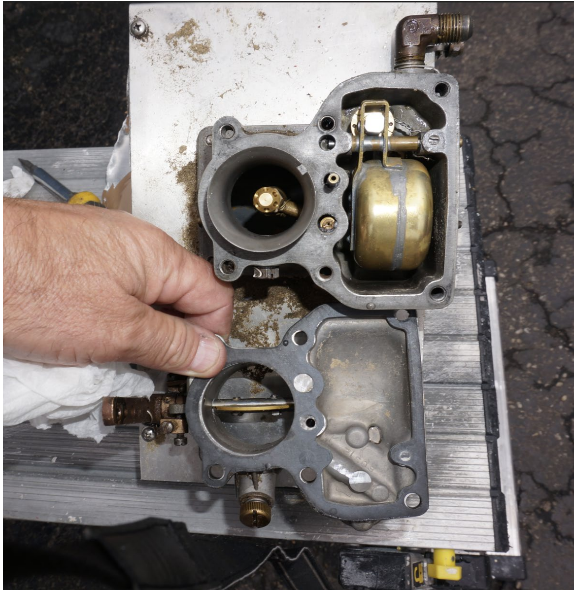
Photograph 7 - Carburetor
