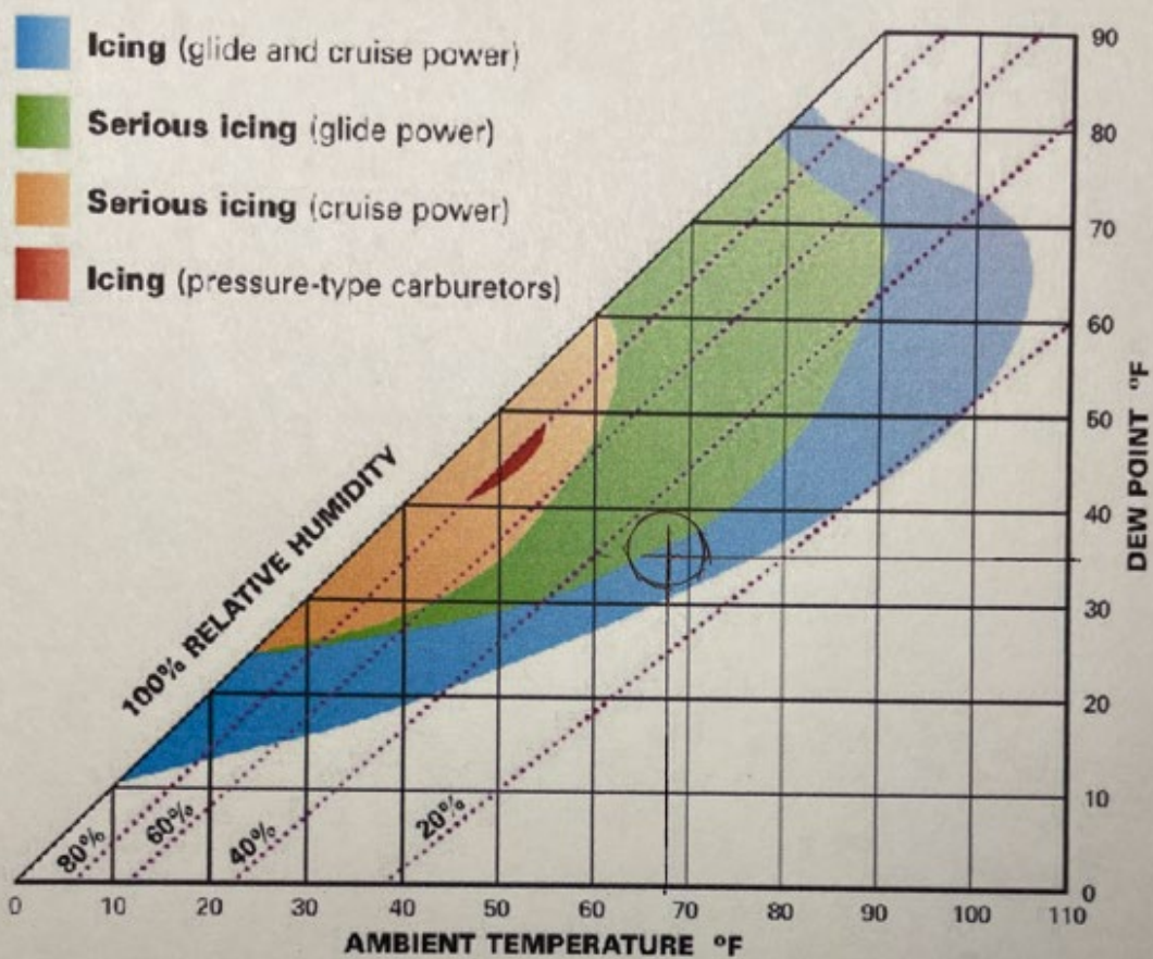
Carburetor Icing Probability Chart
