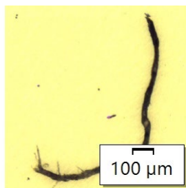
Feret Max.: 920.59 μm Particle Type: Regular Fiber
