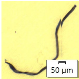
Feret Max.: 674.09 µm Particle Type: Regular Fiber
