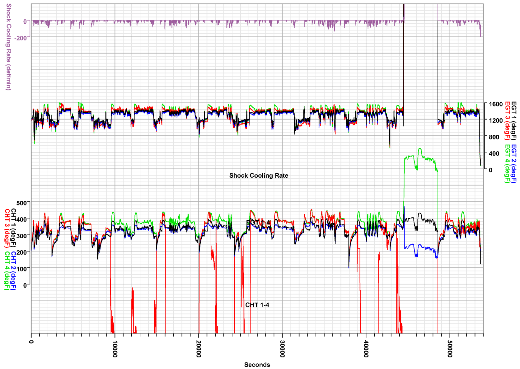
Plot of EGT & CHT parameters for all sessions recorded on the JPI EDM-700.
