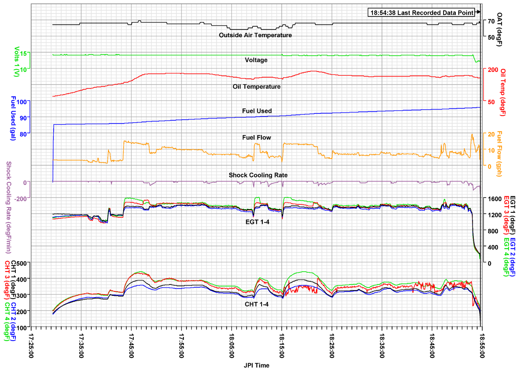
Plot of parameters of the entire last session recorded on the JPI EDM-700.
