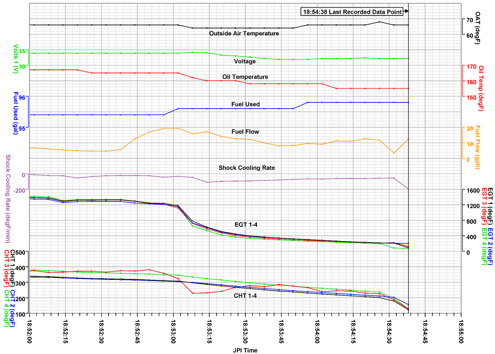
Plot of parameters of the end of the last session recorded on the JPI EDM-700.
