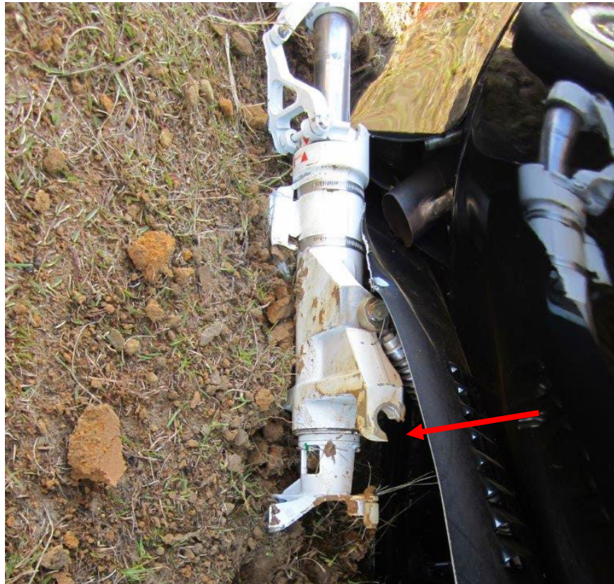
Photograph 5 - Fractured Landing Gear Trunnion (Courtesy FAA)
