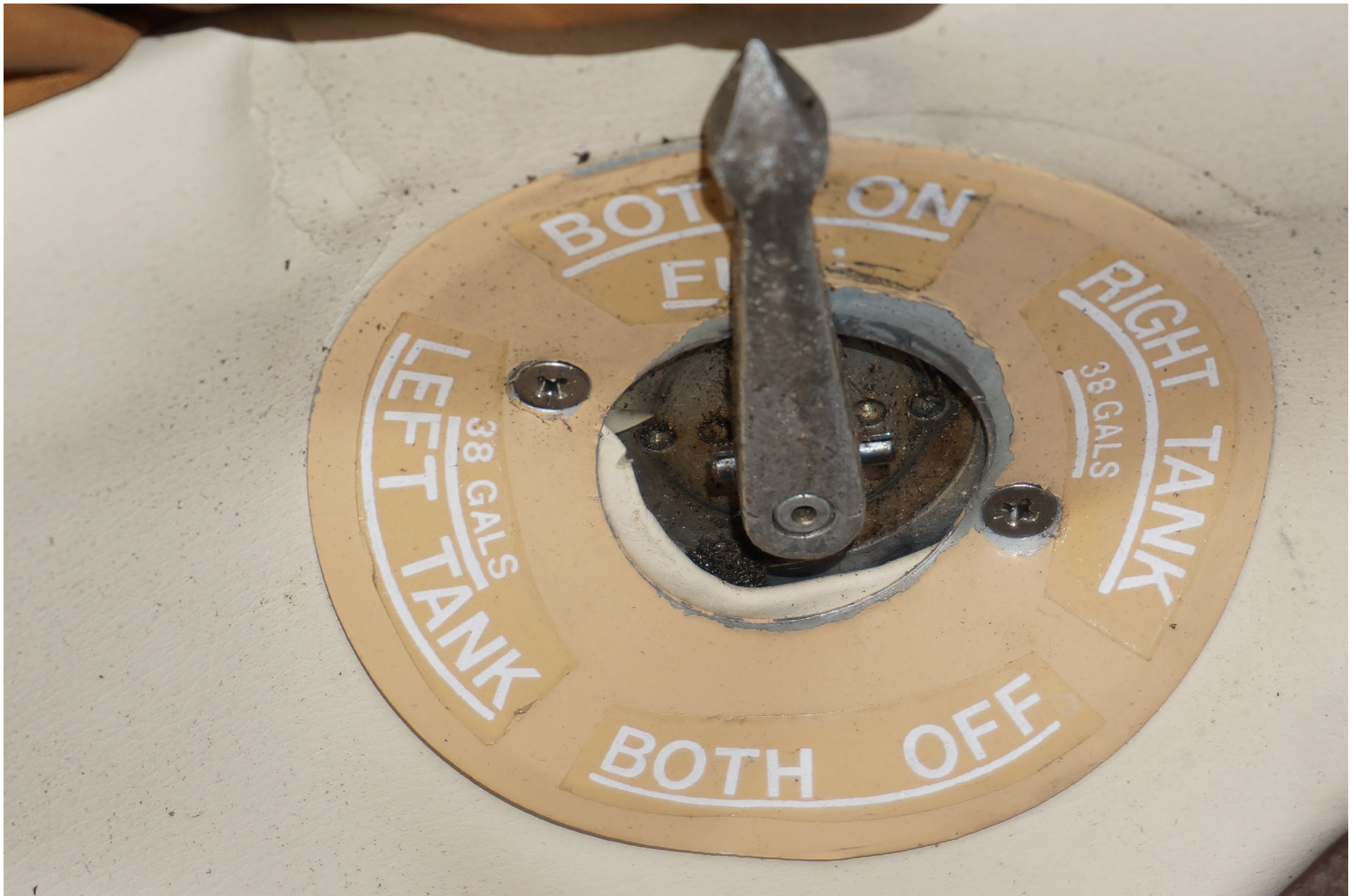
Photo 7 – Fuel Selector
