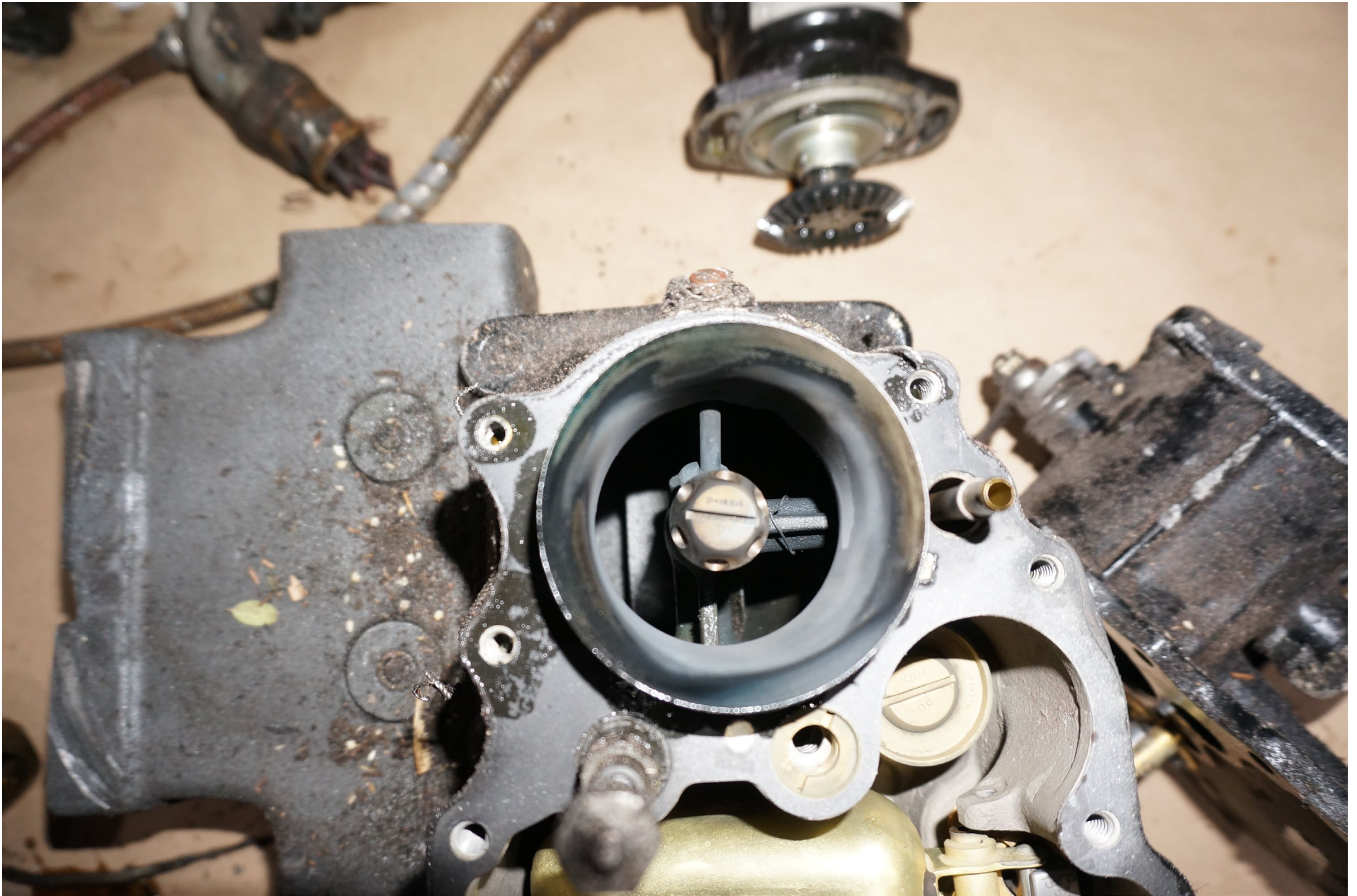
Photo 15 – Carburetor Throat
