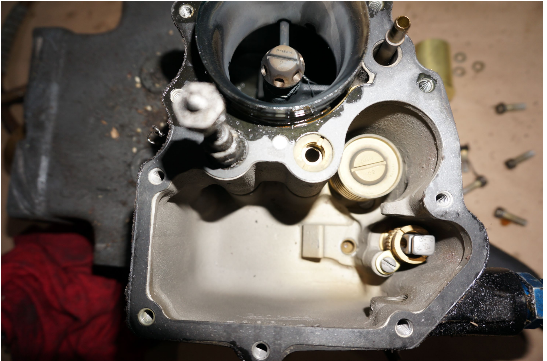
Photo 18 – Carburetor Float Chamber (With Float Removed)
