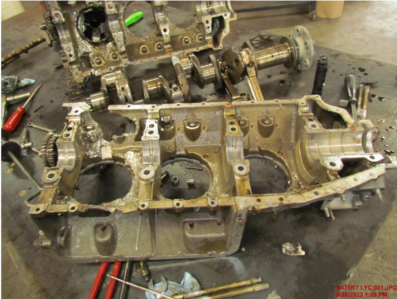
Photograph 3 - Engine crankcase halves separated. (Courtesy of Lycoming)
