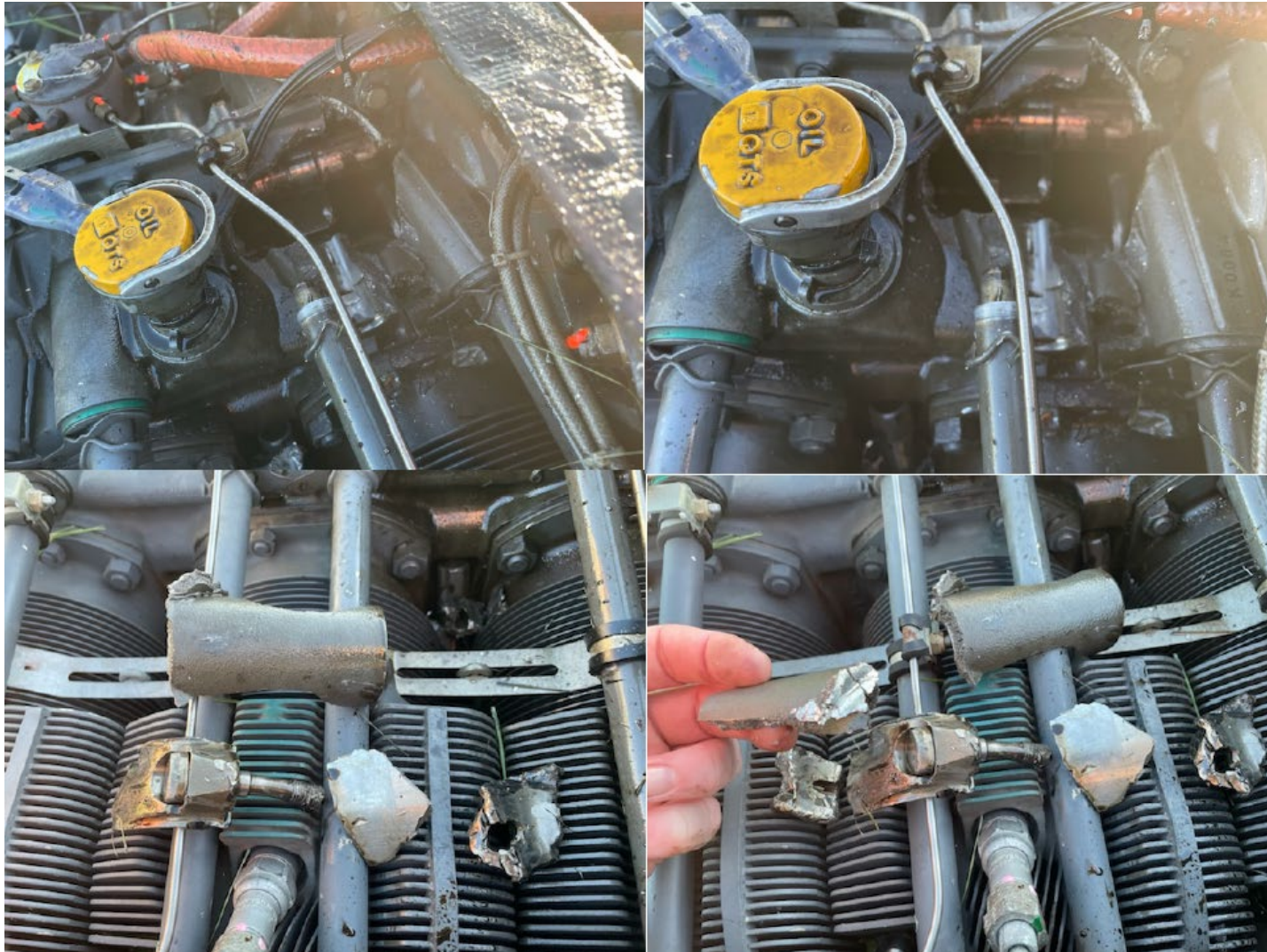
Photograph 4 -Top of engine case showing hole and damaged parts. (Courtesy of FAA)
