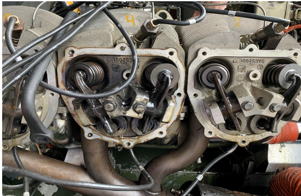
Photos 7, 8, 9: Overview of each cylinder (NTSB Photo)
