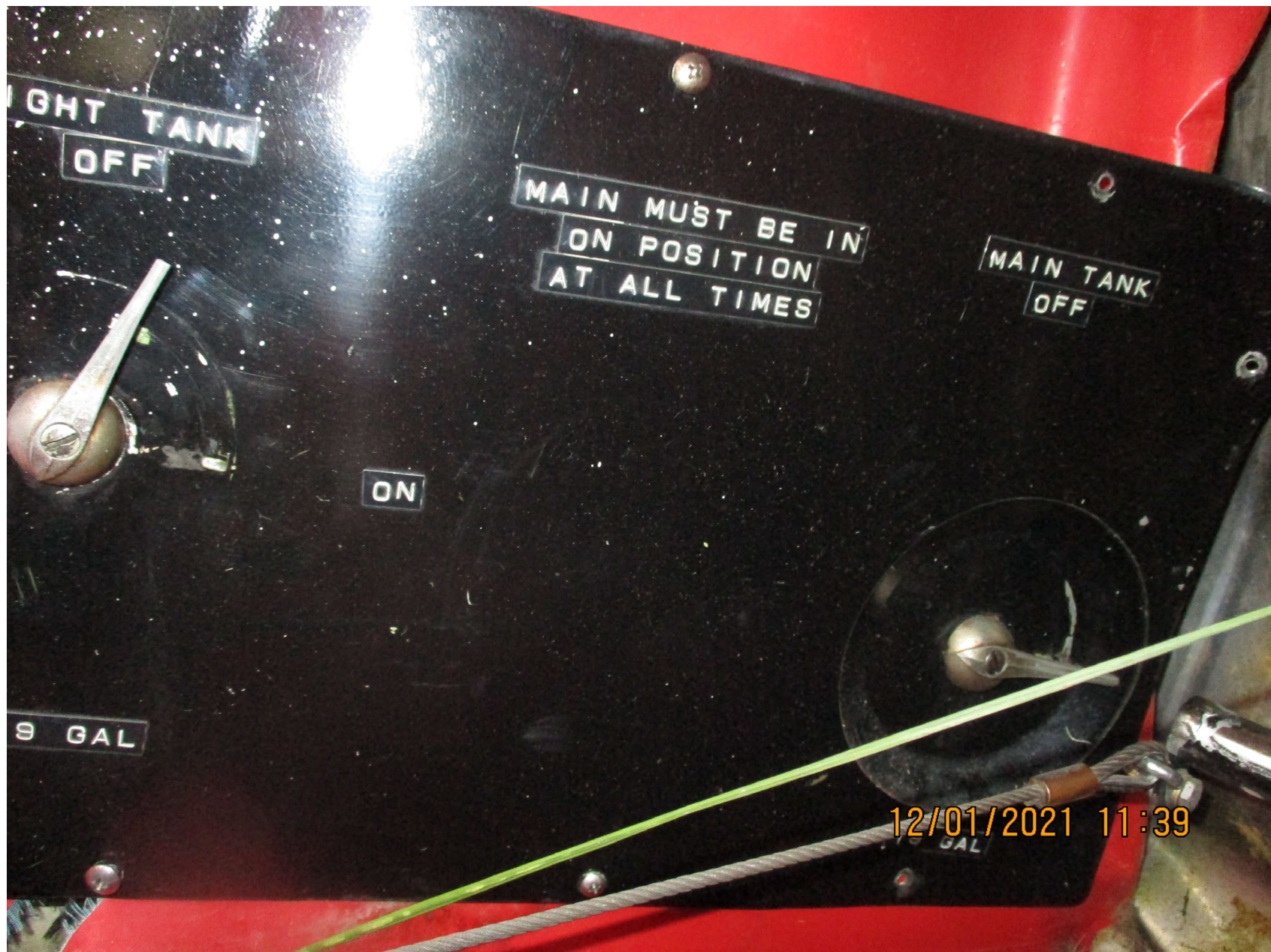
Photo 8 – Fuel Selector Panel – Courtesy of FAA
