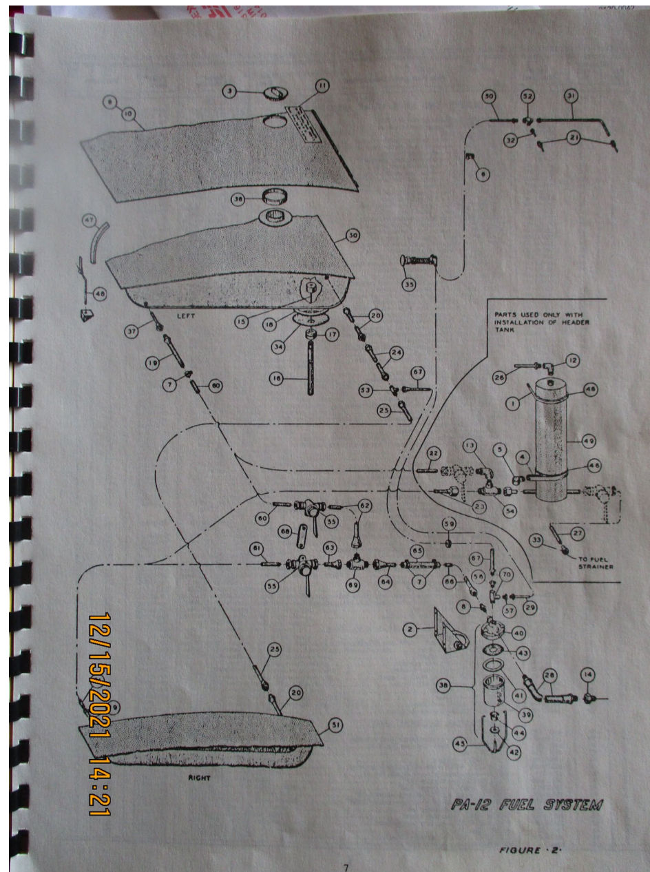
Photo 13 – Fuel System Schematic – Courtesy of FAA
