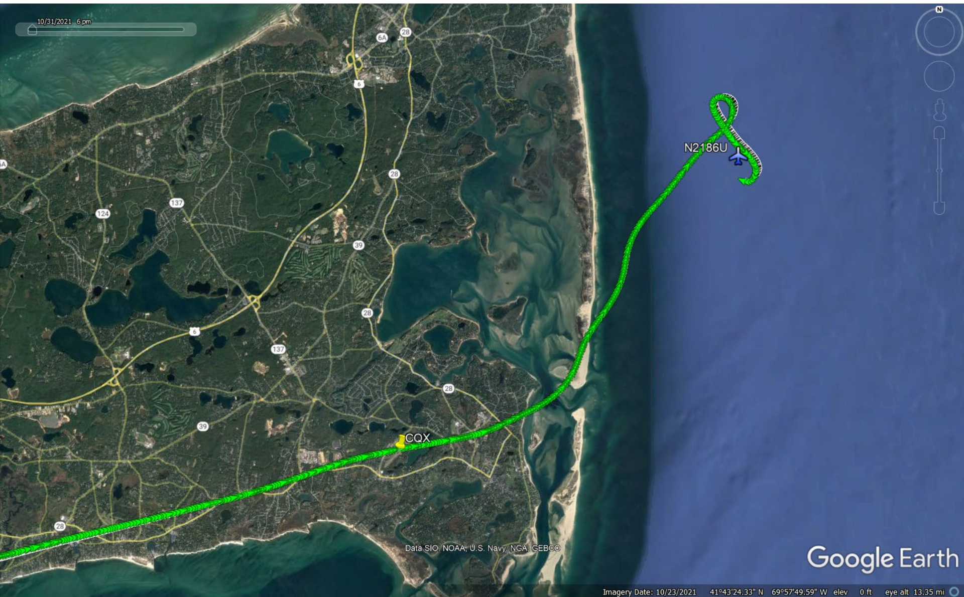
View of final portion of accident flight.
