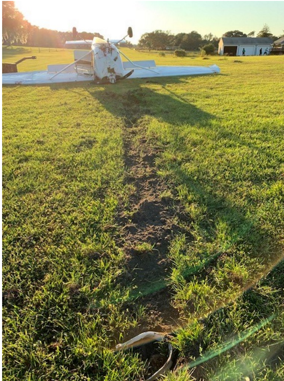
Photo 1 – Airplane at Accident Site Inverted (credit Lake County Sheriff's Office)
