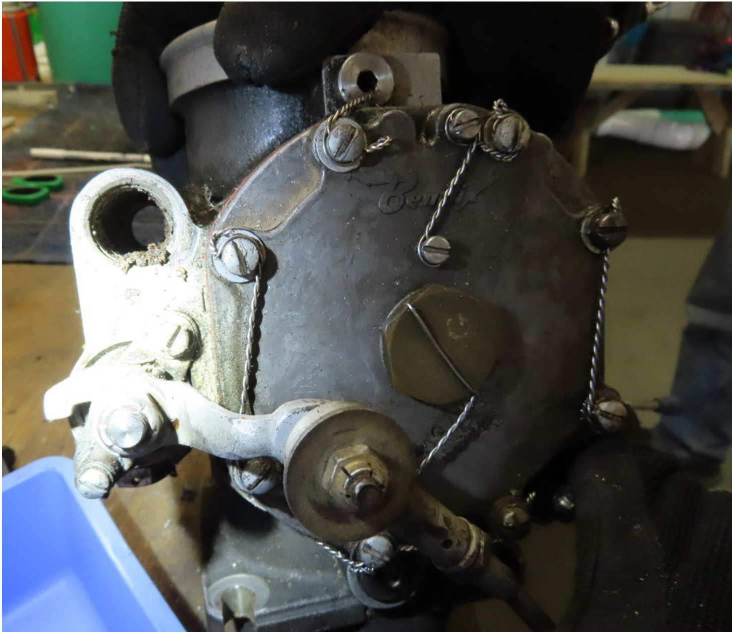
Photo 7 – View of the inlet side of the left fuel servo.
