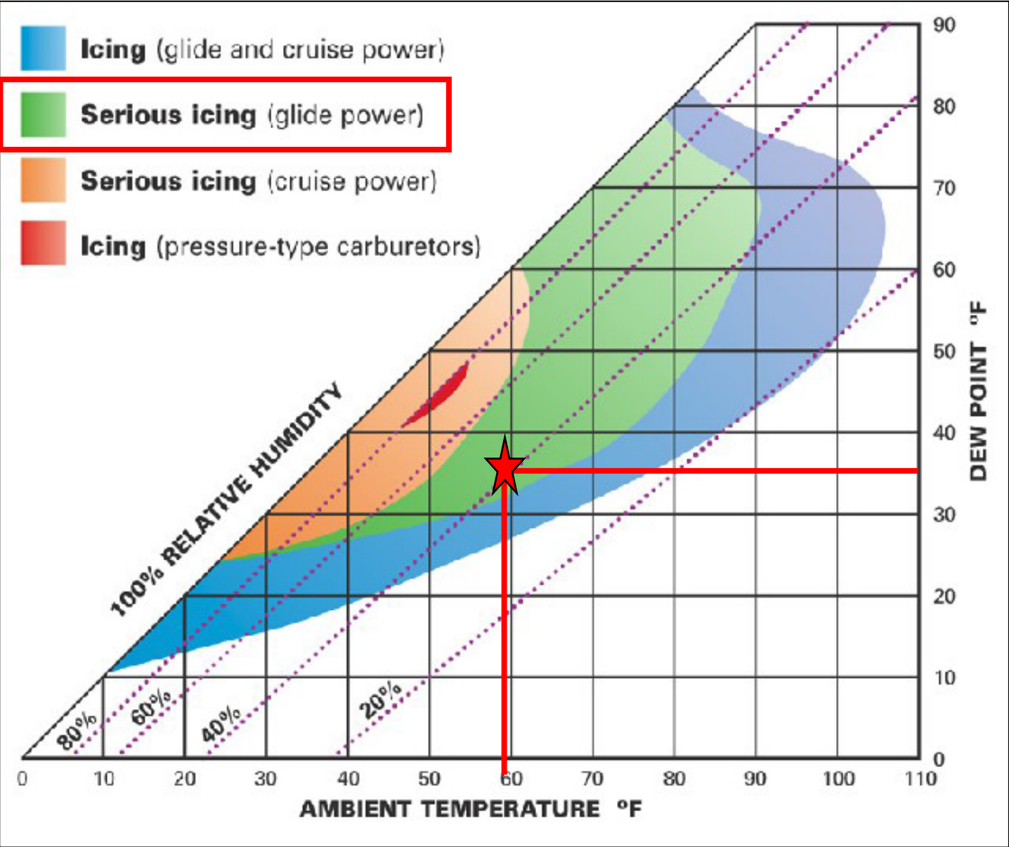
Figure 1 - Carburetor Icing Chart (Source FAA)
