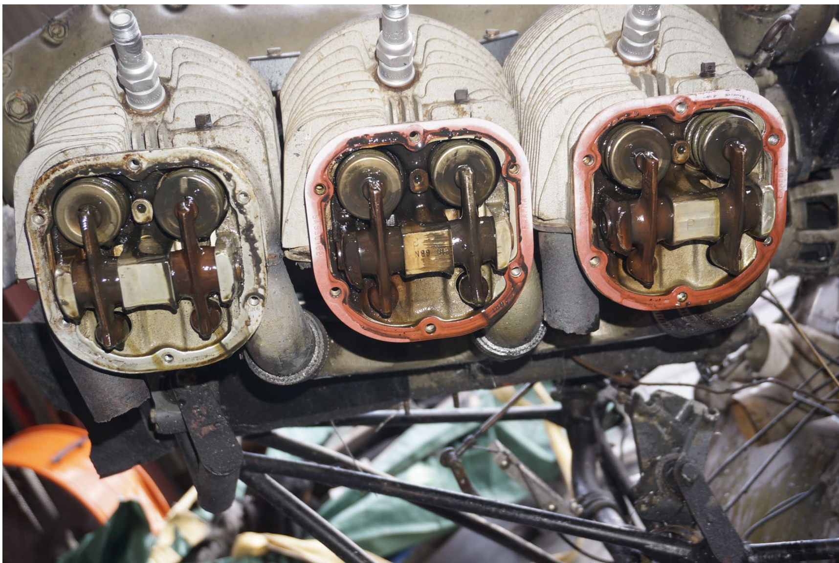
Photograph 27 - Left Cylinder Bank
