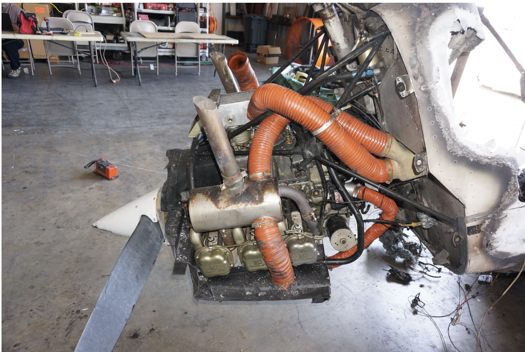
Photograph 16 - Engine
