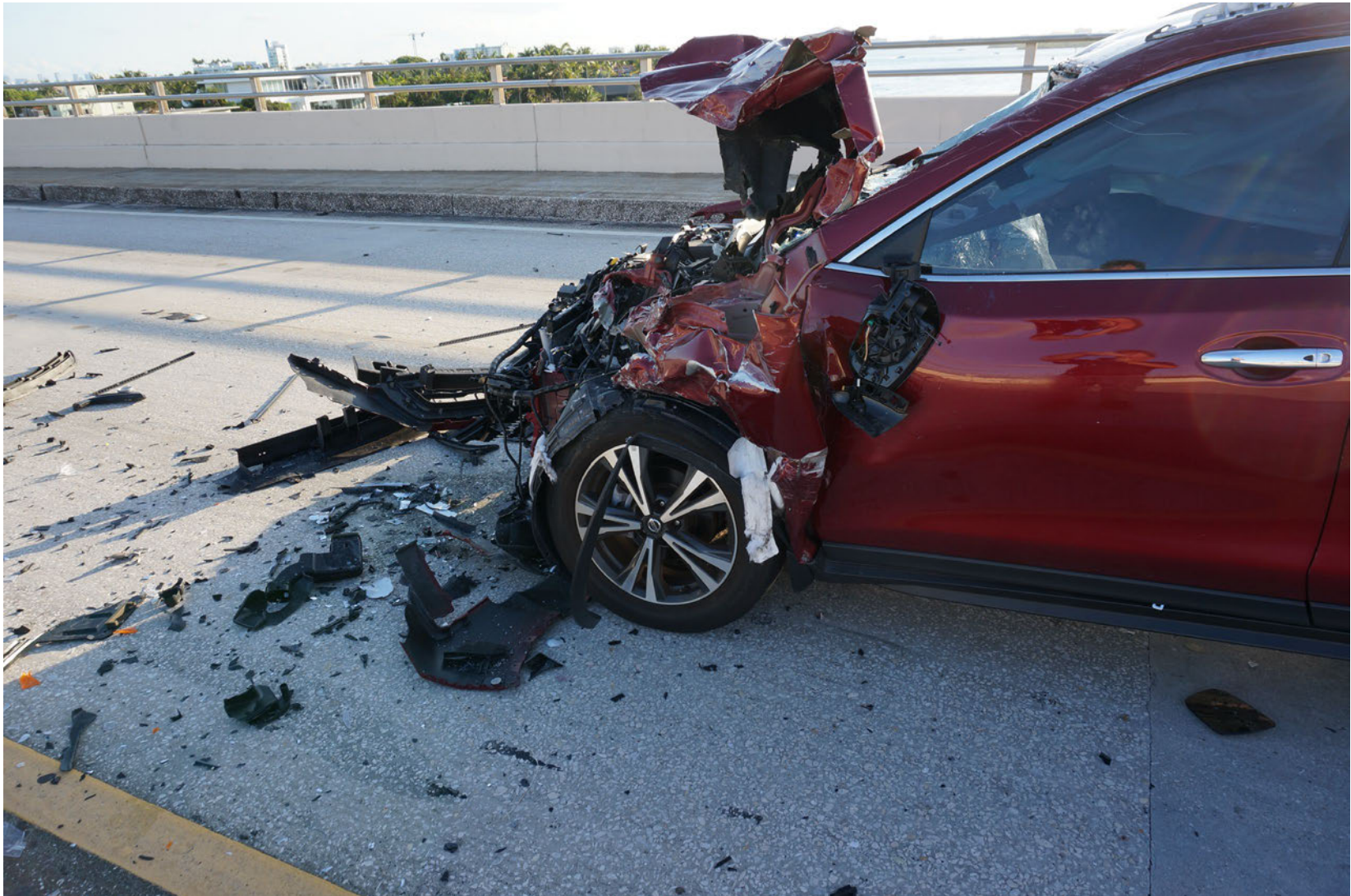
Photograph 3 - Left Side View of Southbound Vehicle
