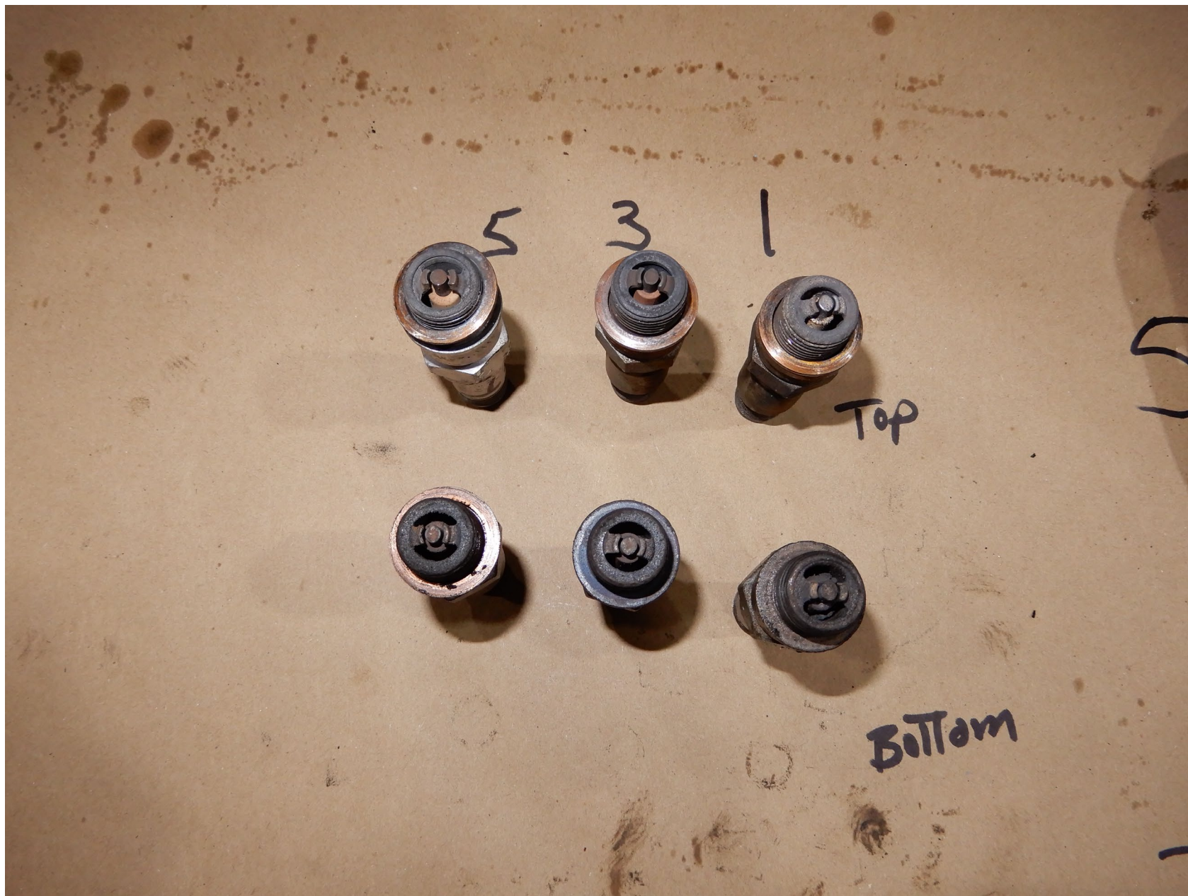
Photo 10 – Spark Plugs (NTSB Photo)
