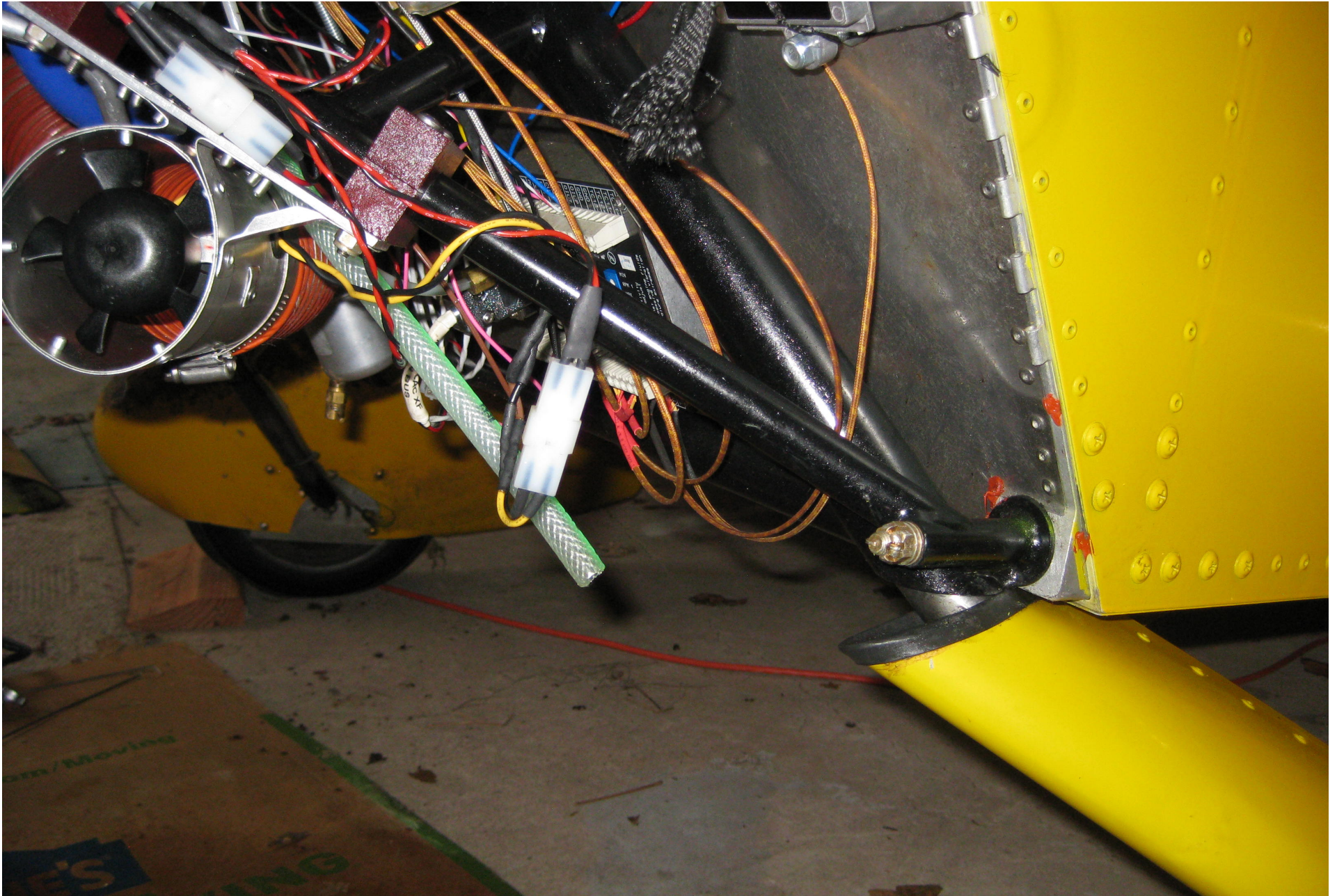
Photo 3 – Landing gear and firewall damage
