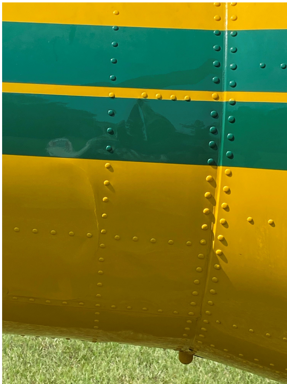
Photo 3 – View of right side showing buckling and cracked paint. (Airbus Photo)
