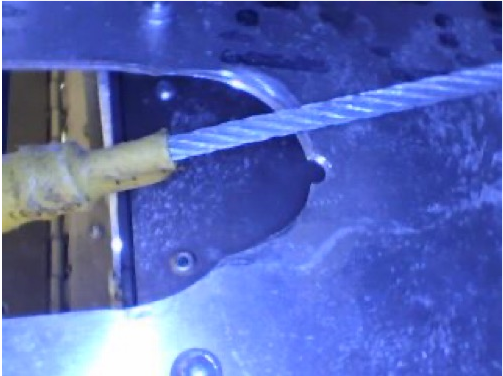
Photo 7– elevator cable cutting into tail section
