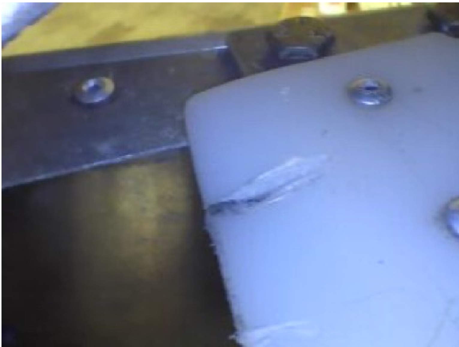
Photo 4– nylon stop with elevator bracket impression marks
