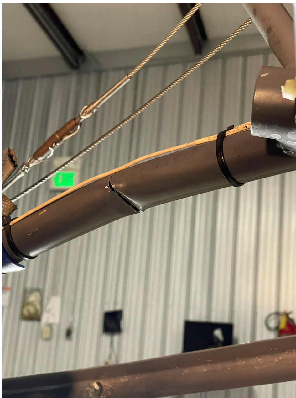
Photo 3 - Digital Photograph From Pilot/Owner. View Depicting Crack and Deformation To One of Four Structural 4130 Steel Tubes That Connect the Tailboom.
