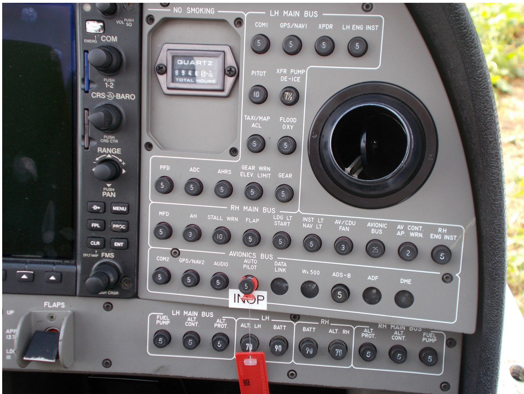
Photo 8 – View of the accident airplane’s circuit breaker panel with the autopilot pulled and collared (Photo Courtesy of FAA)
