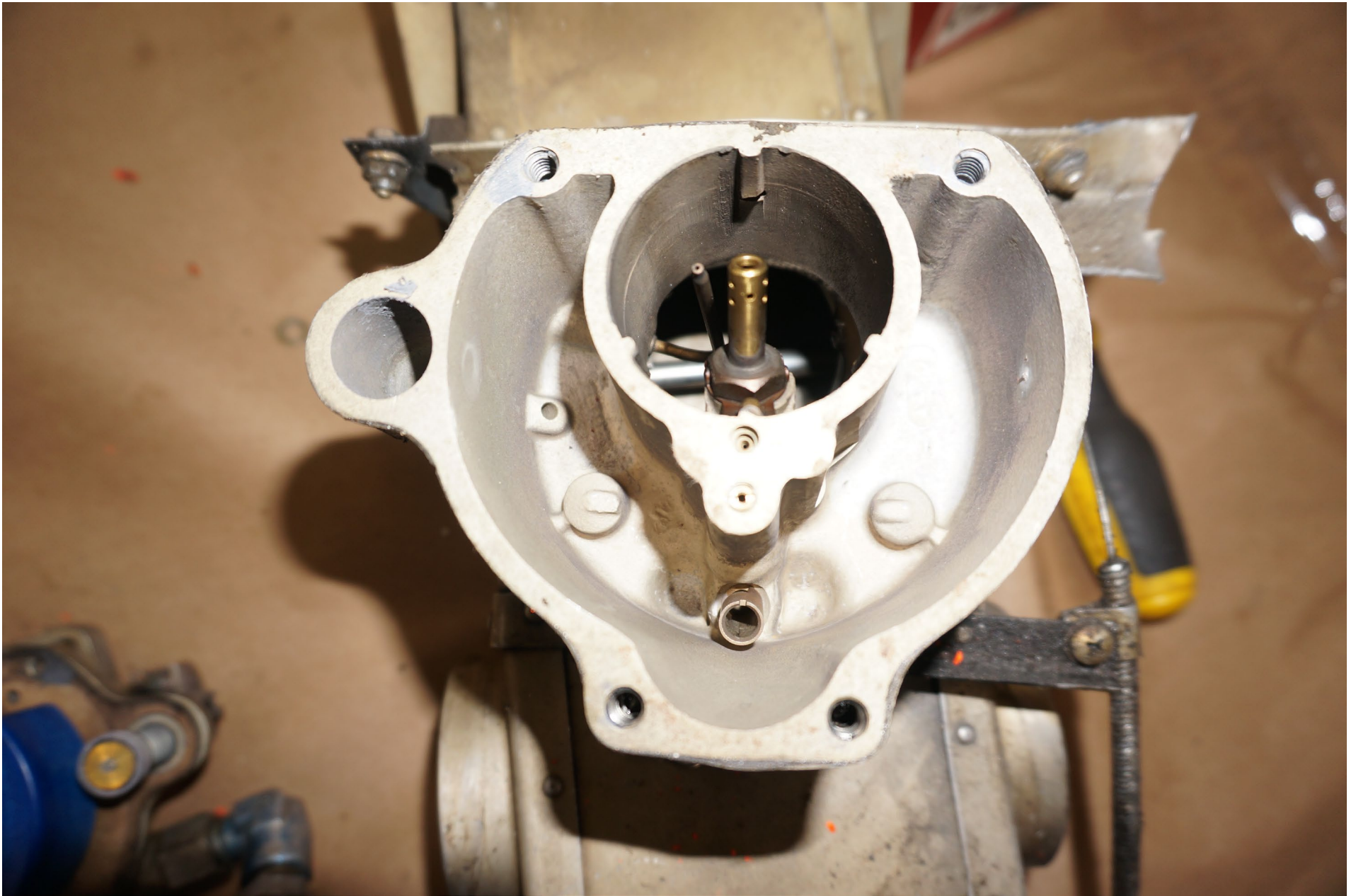
Photo 19 – Interior View of Carburetor Throat and Float Bowl
