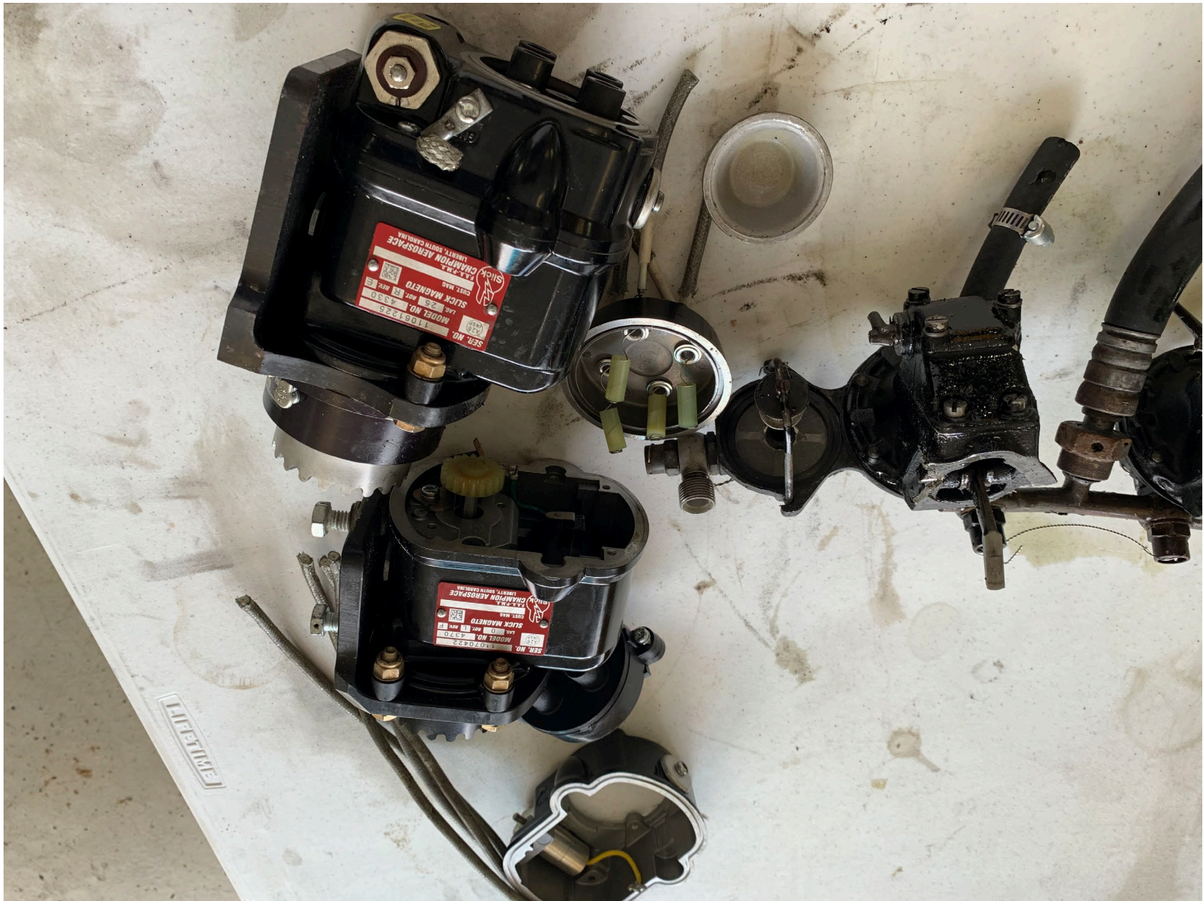
Photo 9 – Magnetos (NTSB Photos)
