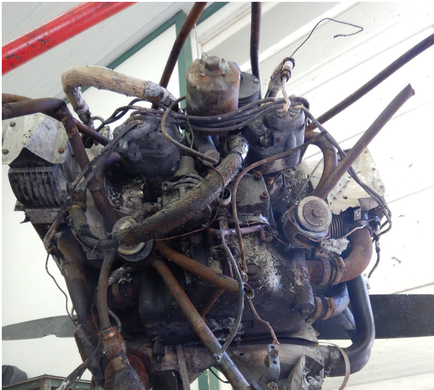
Photo 6 – engine rear view
