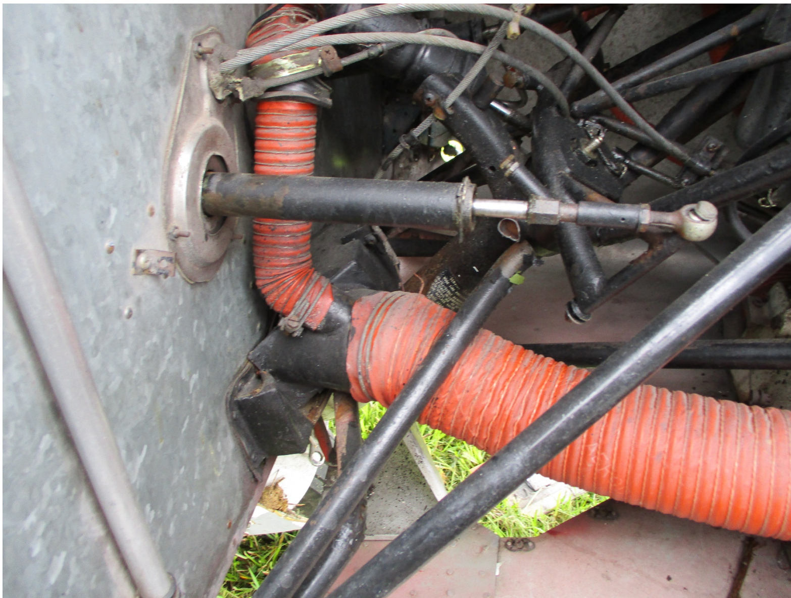
Photo 2 – View of Engine Mount Damage. (Courtesy of FAA)
