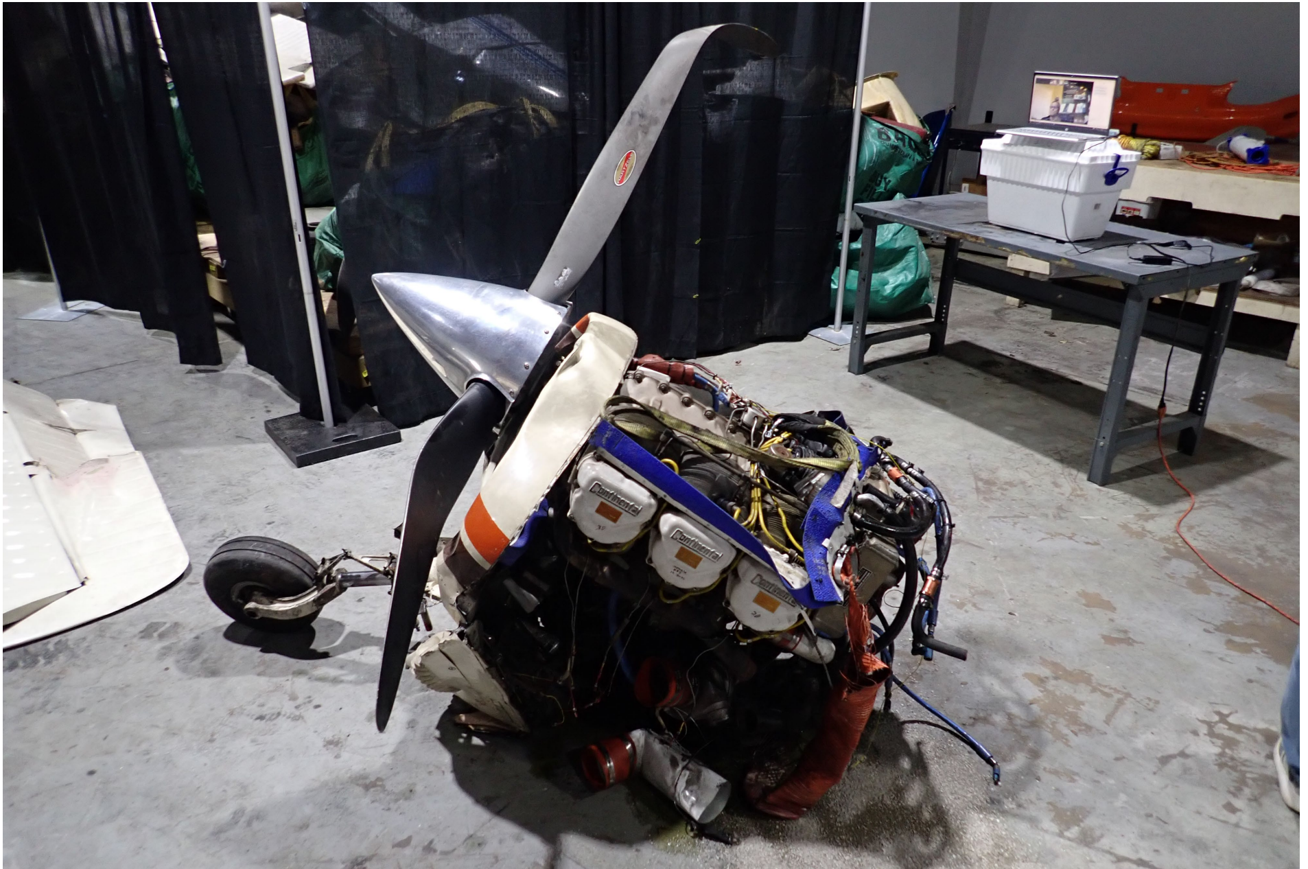
Photo 4 – Textron Aviation Digital Photograph. Left Side View of the Engine Assembly with Attached Propeller Following Recovery. Note the Minimal Bending of Both Propeller Blades.
