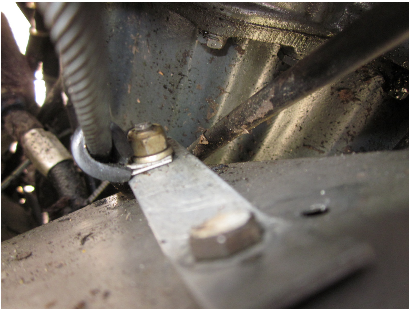
Photo 8 - Throttle Cable and Standoff Clamp After Repositioning – Courtesy of FAA
