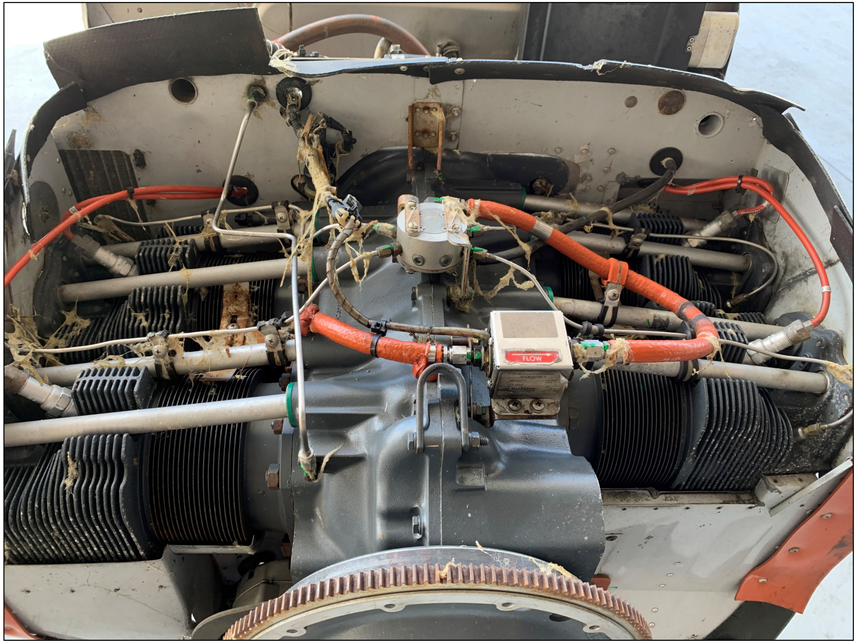
Photo 3 – Overview of the engine
