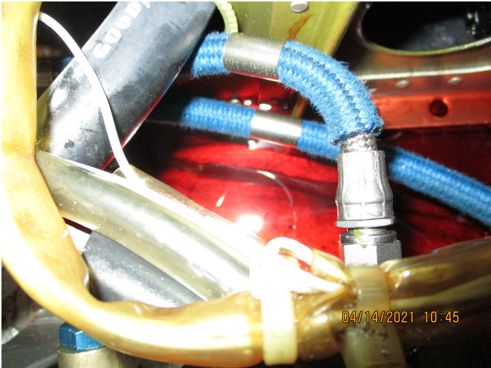
Photo 3 – Left main landing gear down and lock actuator, leaking
