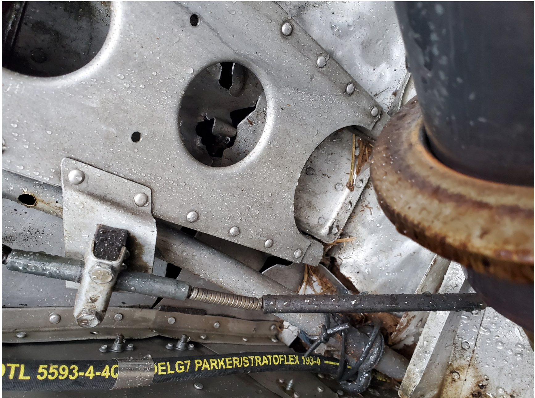
Photo 4 – cracked structure (FAA)
