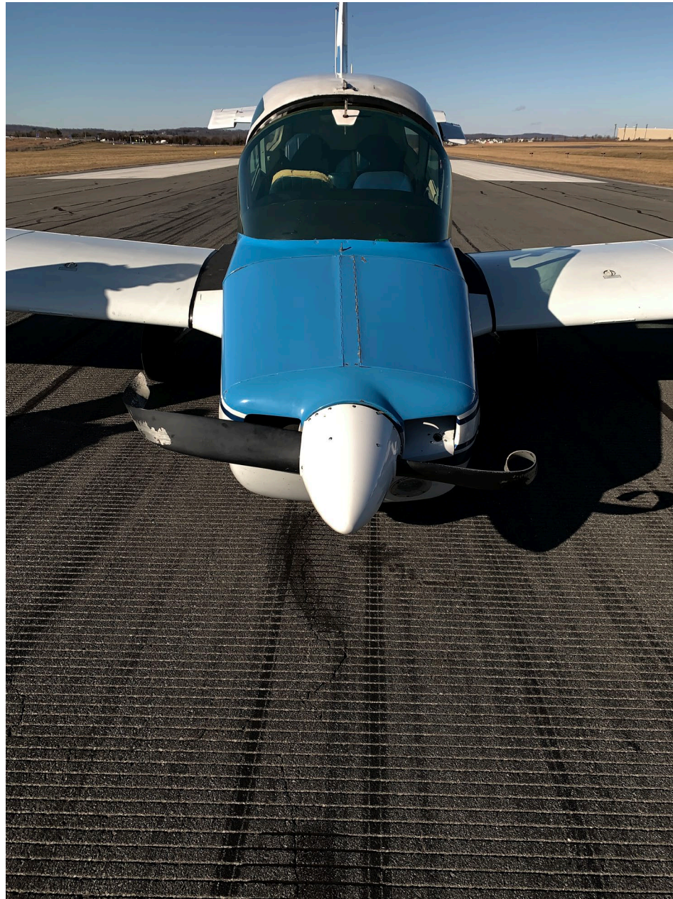
Photo 1 – FAA Digital Photograph. Frontal View of the Airplane on the Runway. Note the collapsed Nose Landing gear.
